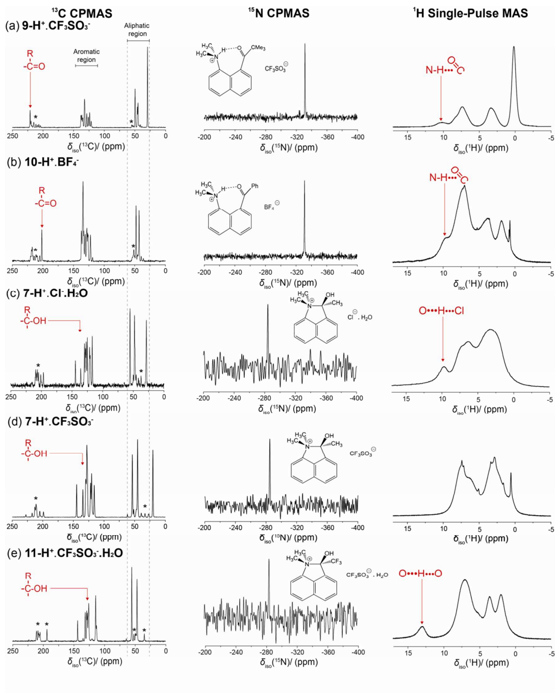
Figure 6. ^{13}\text{C} , ^{15}\text{N} and ^1\text{H} CPMAS NMR spectra for salts 9\text{-H}^+\cdot\text{CF}_3\text{SO}_3^- and 10\text{-H}^+\cdot\text{BF}_4^- (upper) and the salts 7\text{-H}^+\cdot\text{Cl}\cdot\text{H}_2\text{O} , 7\text{-H}^+\cdot\text{CF}_3\text{SO}_3^- and 11\text{-H}^+\cdot\text{CF}_3\text{SO}_3^-\cdot\text{H}_2\text{O} (lower).
