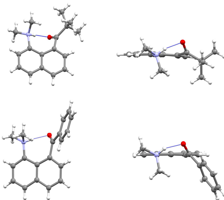
Figure 5: Two views of the molecular structure and intramolecular hydrogen bond of (a) one of the two independent cations of 9-H + (top), (b) the cation 10-H + (bottom).
