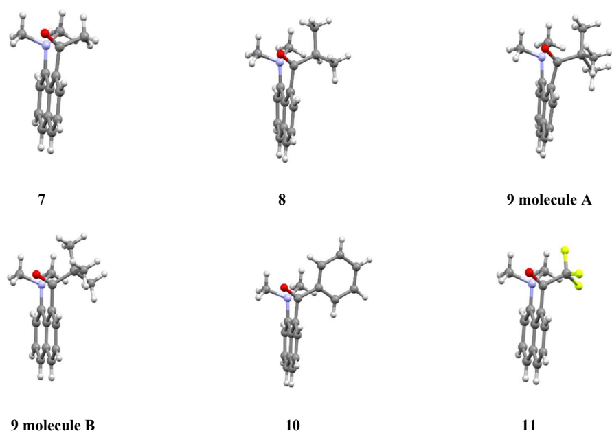
Figure 1. Molecular structures of the ketone 7-11 , showing the increase in displacements from the naphthalene plane as the Me 2 N...C=O separation increases (top row), but the
