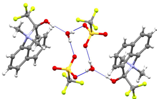
Figure 3. Hydrogen bonding linking together two cations with a cluster of two triflate anions and two water molecules in the crystal structure of 11\text{-H}^+\cdot\text{triflate}\cdot\text{H}_2\text{O} .
