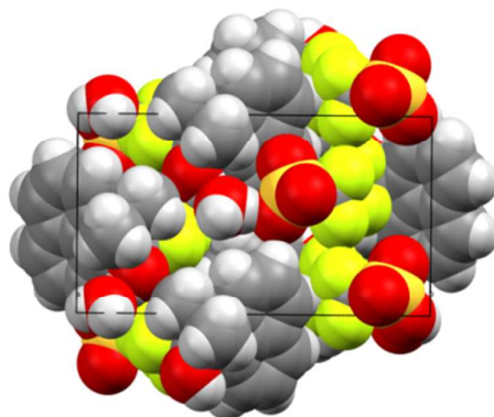
Figure 4. Space-filling view of the crystal packing of 11-H + .triflate.H 2 O viewed down the a axis, showing the segregation of the fluororous residues.
