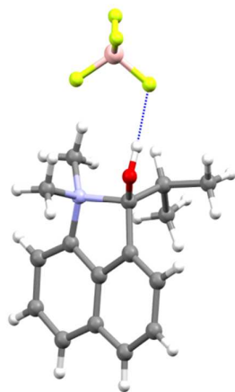
Figure 2. Molecular structures of (a) the hydrated chloride salt of the O-protonated methyl ketone 7\text{-H}^+ showing the involvement of anions and water molecules in the hydrogen bonding pattern (left), (b) the triflate salt of 7\text{-H}^+ (right) and (c) the tetrafluoroborate salt of the O-protonated isopropyl ketone 8\text{-H}^+ (below).
