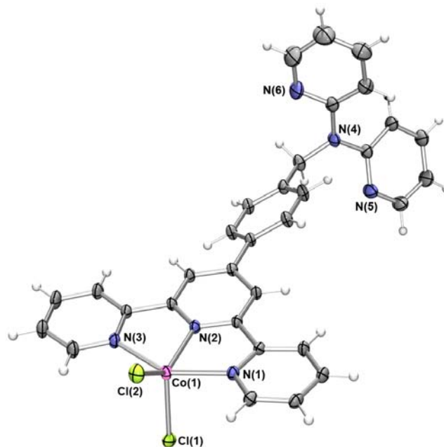
Fig. 1 X-ray structure of [CoLCl 2 ]·0.25DCM·0.5H 2 O. Solvent molecules have been removed for clarity. Thermal ellipsoids are shown at the 50 percent probability level.
