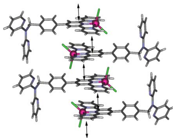
Fig. 2. Representation of the one-dimensional stack that propagates parallel to the crystallographic ab vector in [CoLCl 2 ]·0.25DCM·0.5H 2 O. Double headed arrows indicate the presence of arene-arene interactions.
