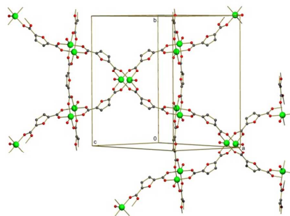
Fig. 2 Infinite two-dimensional coordination layer in the crystal structure of Cu-FDC. Hydrogen atoms are omitted for clarity.
