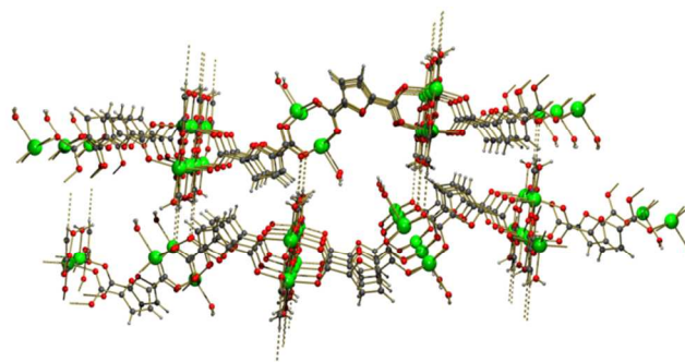
Fig. 3 Weak C-H...O hydrogen bonding in the crystal structure of Cu-FDC. Viewed along the crystallographic b -axis. Two-dimensional coordination planes are shown horizontally. Hydrogen bonds are shown as dashed lines.
