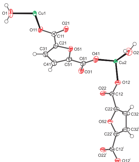
Fig. 1 Asymmetric unit of the crystal structure of Cu-FDC. Viewed along the crystallographic c -axis. Displacement ellipsoids are drawn at the 50% probability level. Atoms Cu1, O1, and O52 are located on crystallographic mirror planes. Non-coordinated solvent molecules were treated as diffuse electron density (see Experimental Section) and were omitted in the drawing. Symmetry operation i : x , - y , z .
