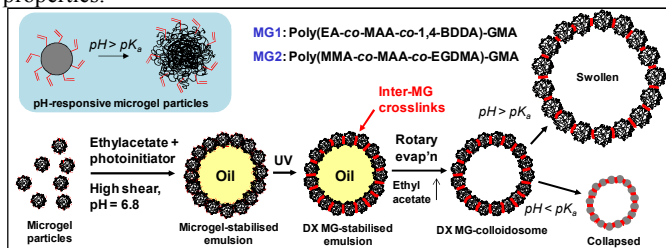
Scheme 1. Illustration of DX MG-colloidosome preparation using pH-responsive microgel particles. The majority of the data presented in this study used MG1 particles. MG2 particles were used to demonstrate versatility.
