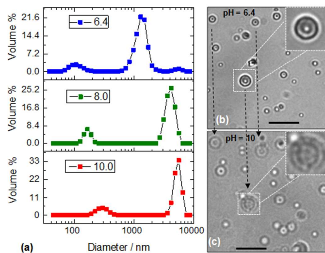
Fig. 3. DLS data measured at various pH values (a) for DX MG-colloidosomes. (b) and (c) show optical micrographs at pH = 6.4 and 10, respectively. The arrows show colloidosomes that did not change position when the pH increased. Scale bar = 10 \mu\text{m} . MG1 particles were used for these colloidosomes.
