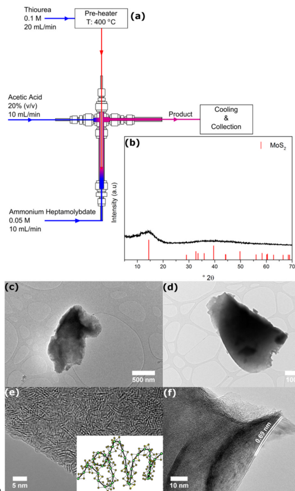
Fig. 2. Reactor for the production of MoS 3 by acidification of in-situ generated thiomolybdates (a), and the XRD pattern (b) and HRTEM images (c-f) of the amorphous product (inset shows a possible structure as proposed by Hibble et al. ).
