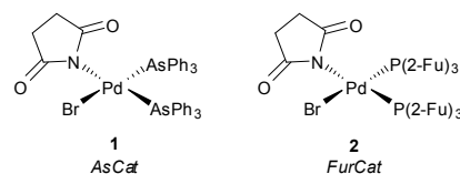
Figure 1 Structures of the two novel succinimide-based catalysts, 1 and 2 .
