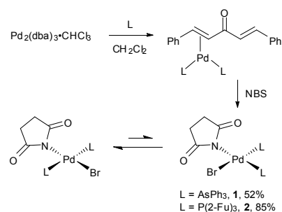
Scheme 1 Synthesis of complexes 1 ( AsCat ) and 2 ( FurCat ).
