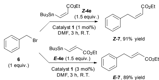
Scheme 1 Coupling of benzyl bromide ( 6 ) with electron deficient stannanes E- and Z-4e using catalyst 1 .
