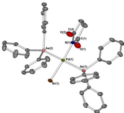
Figure 2 The crystal structure of complex 1 . Hydrogen atoms have been removed and only selected atoms are numbered for clarity. Thermal ellipsoids are shown with a probability of 50%. Selected bond lengths (Å): Pd(1)–As(1): 2.4229(4), Pd(1)–Br(1): 2.4338(4), Pd(1)–As(2): 2.3914(4), Pd(1)–N(1): 2.025(2). Selected bond angles (°): N(1)–Pd(1)–As(1): 90.69(7), As(1)–Pd(1)–Br(1): 92.969(13), Br(1)–Pd(1)–As(2): 87.471(13).
