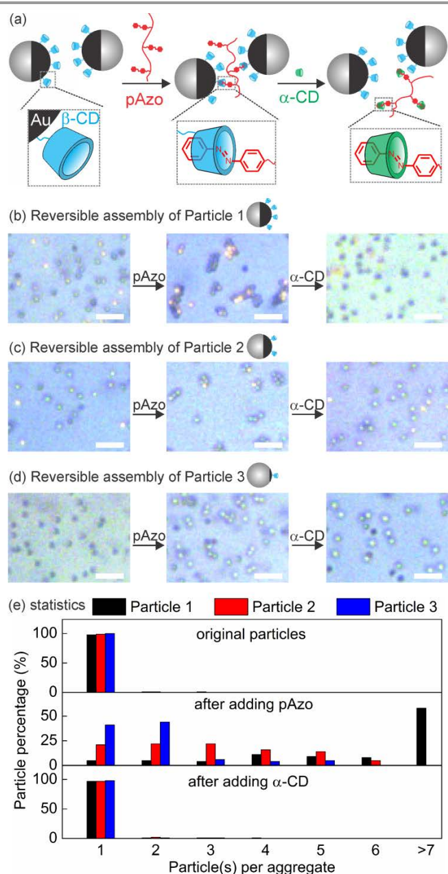
Fig. 2 (a) Schematic illustration of reversible assembly of \beta -CD-modified Janus particles by sequential addition of azobenzene-containing polymer (pAzo) and \alpha -CD. (b)-(d) Optical microscopy images: reversible assembly of Particle 1 (b), Particle 2 (c), and Particle 3 (d). The time for assembly and disassembly is 84 s and 105 s, respectively. The scale bar is 5 \mu m. Corresponding movies are provided in ESI † . (e) Number distribution of Janus particle aggregates consisting of different numbers of particles in the reversible assembly processes. The statistical results are obtained from \sim 400 particles.
