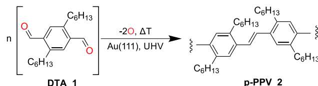
Fig. 1 Investigated on-surface reaction.
