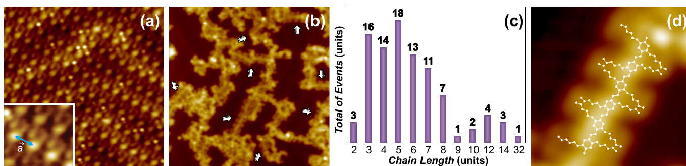
Fig. 2 Deposition and on-surface reaction of DTA monomers on Au(111). a) STM image ( 12 \times 12 \text{ nm}^2 ; U = -1.50 \text{ V} ; I = 400 \text{ pA} ) after the deposition onto the surface kept at room temperature. The inset shows the intermolecular distance between adjacent monomers along the aldehyde moiety direction. b) STM image ( 30 \times 30 \text{ nm}^2 ; U = -0.65 \text{ V} ; I = 7 \text{ pA} ) after the deposition onto the surface kept at 250 \text{ }^\circ\text{C} . The targeted coupling reaction is achieved, producing p-PPV oligomers (white arrows) on the surface. c) Oligomers 2 chain length distribution. d) High resolution STM image ( 5.7 \times 8.5 \text{ nm}^2 ; U = 0.65 \text{ V} ; I = 7 \text{ pA} ) of the p-PPV products 2 . The inset schematically represents the chemical structure of the reacted specie.
