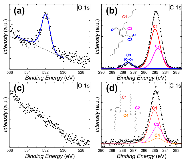
Fig. 3 XPS analysis of the on-surface reaction. a-b) XPS data of the C1s and O1s regions after deposition onto the substrate kept at room temperature. Peak fitting analysis reproduced the stoichiometry of intact monomers. c-d) XPS data collected after the deposition onto the substrate kept at 250 °C show a complete absence of oxygen species. The C1s signal is consistent with the formation of p -PPV 2 , but does not exclude contributions from oxygen-free side products in the disordered phase.
