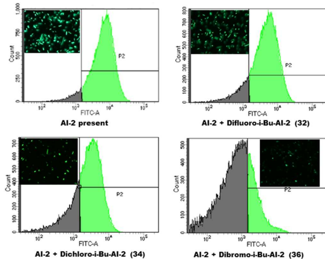
Figure 5. AI-2 dependent EGFP induction in E. coli W3110 pCT6( luxS + ) in response to difluoro-iBu-AI-2 (32), dichloro-iBu-AI-2 (34) and dibromo-iBu-AI-2 (36) (FACS analysis with microscopic image).
