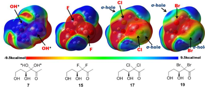
Figure 6. Molecular surface electrostatic potential of AI-2 and analogs in simplified models. Color ranges from -9.5 kcal/mol (red) to 9.5 kcal/mol (blue). Important atoms and \sigma -hole are labeled.
