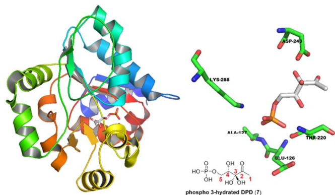
Figure 3. Phospho-AI-2 in its hydrated form at C3 when binding with LsrR (PDB code: 4L4Z). Asp243 is 2.7 Å from geminal diol unit of phospho-AI-2.
