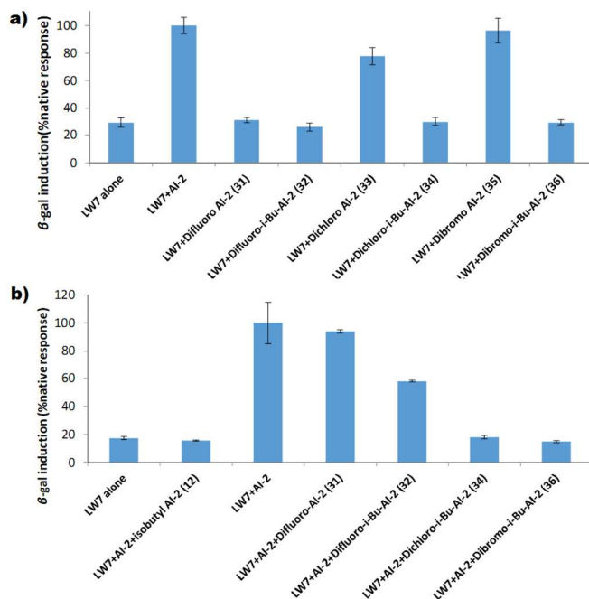
Figure 4. a) AI-2 dependent \beta -galactosidase production of E. coli LW7 ( luxS ) in response to 20 \mu M synthetic AI-2 or analogs. b) Analogs (20 \mu M) inhibit native \beta -galactosidase production in E. coli LW7 ( luxS ) in the presence of 20 \mu M synthetic AI-2.
