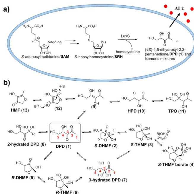
Figure 1 a) Biosynthesis of AI-2. b) Chemical structures of AI-2.
