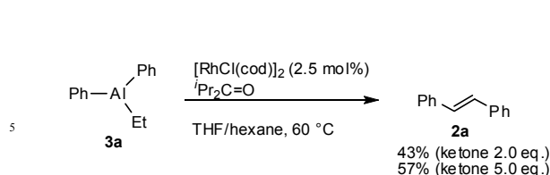
Scheme 2. Rhodium catalyzed reaction of diethyl(phenyl)aluminum
