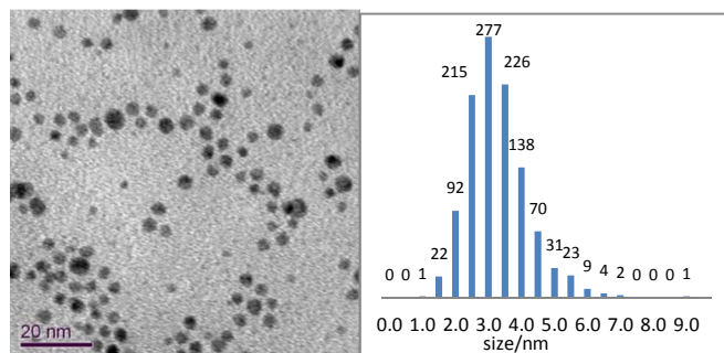
Fig. 4. TEM image of arsonium-AuNP derived from zwitterion 3 and associated particle size histogram.
