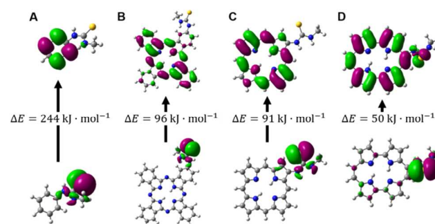
Fig. 4 HOMO-LUMO energy gap ( \Delta E = E_{\text{LUMO}} - E_{\text{HOMO}} ) of different aromatic thioureas, namely, (A) N -methyl- N' -phenylthiourea, (B) N -methyl- N' -(2-phthalocyanine)-thiourea, (C) N -methyl- N' -(2-porphyrin)-thiourea, and (D) N -methyl- N' -(9-porphycene)-thiourea
