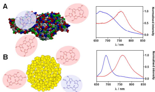
Fig. 2 Fluorescence spectra of unbound 9-ITPPo (blue) and its covalent adduct ATAZPo (red) with BSA (A) and AuNCs (B).
