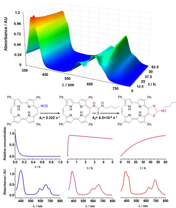
Fig. 3 Top: Time evolution of the absorbance of a mixture of 9-ITPPo (15 \mu\text{M} ) and n -butylamine (3 mM) in toluene. Bottom: Structures, concentration evolution and spectral profiles of the reactant, the intermediate and the product (from left to right) achieved through singular value decomposition of the spectral evolution in air.
