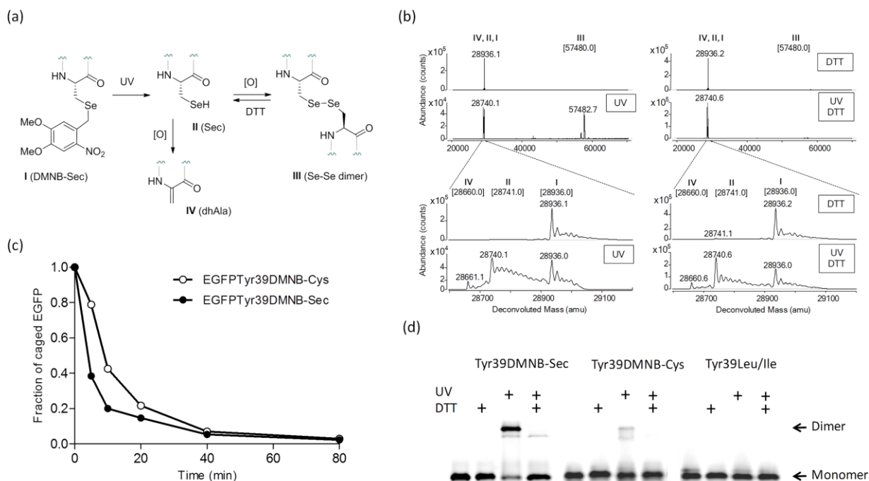
Fig. 2 Photochemical decaging of the EGFP-Tyr39DMNB-Sec protein. (a) Transformations of the incorporated DMNB-Sec residue (I) to selenocysteine (II) diselenide dimer (III) or dehydroalanine (IV). (b) ESI-MS analysis of photolysis products before (upper) and after 20 min exposure (lower) of isolated EGFP-Tyr39DMNB-Sec protein to UV light. Photodecaging reactions were performed under non-reducing (left) or reducing (DTT, right) conditions. Samples were resolved on an Agilent 1290 Infinity HPLC system equipped with a Poroshell 300SB-C8 column by elution with 1% formic acid in a gradient of water/acetonitrile at a flow rate of 0.4 ml/min. High-resolution mass spectra were acquired on an in-line Agilent Q-TOF 6520 mass analyzer (100–3200 m/z range, positive ion mode) and analyzed with MassHunter software. Theoretical masses of EGFP variants I–IV are shown in brackets. ‡ (c) Representative time courses of photochemical decaging under reducing conditions analyzed by HPLC/ESI-MS (Fig. S2†). (d) Semi-native SDS-PAGE gel analysis of fluorescent EGFP variants (EGFP-Tyr39DMNB-Sec, EGFP-Tyr39DMNB-Cys, and EGFP-Tyr39Leu/Ile) before and after UV illumination (UV) under non-reducing and reducing (DTT) conditions.
