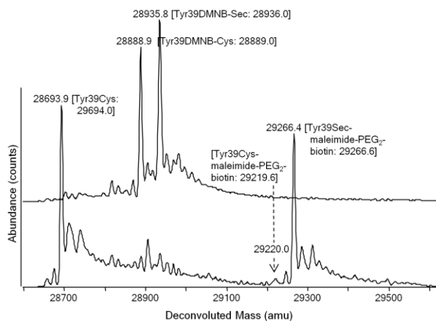
Fig. 3 Selective labeling of a Sec-containing EGFP with a maleimide probe. HPLC/ESI-MS analysis of an equimolar mixture of DMNB-caged EGFP-Tyr39Sec and EGFP-Tyr39Cys proteins (upper) and following its UV-illumination and treatment with maleimide-PEG 2 -biotin (lower) under reducing and slightly acidic conditions (pH 5.0). Analysis was performed as described in Fig. 2b. Deconvoluted spectrograms are scaled to a signal intensity of the most abundant peak ( 8.5 \times 10^5 counts). Theoretical masses are shown in brackets.
