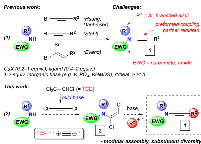
Scheme 1. Copper-catalyzed ynamide formations, and the planned modular approach to ynamides 1 via dichloroamides 2 .
