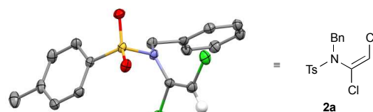
Figure 1. ORTEP diagram for ( E )-dichloroenamide 2a (the alkene hydrogen is retained for clarity).
