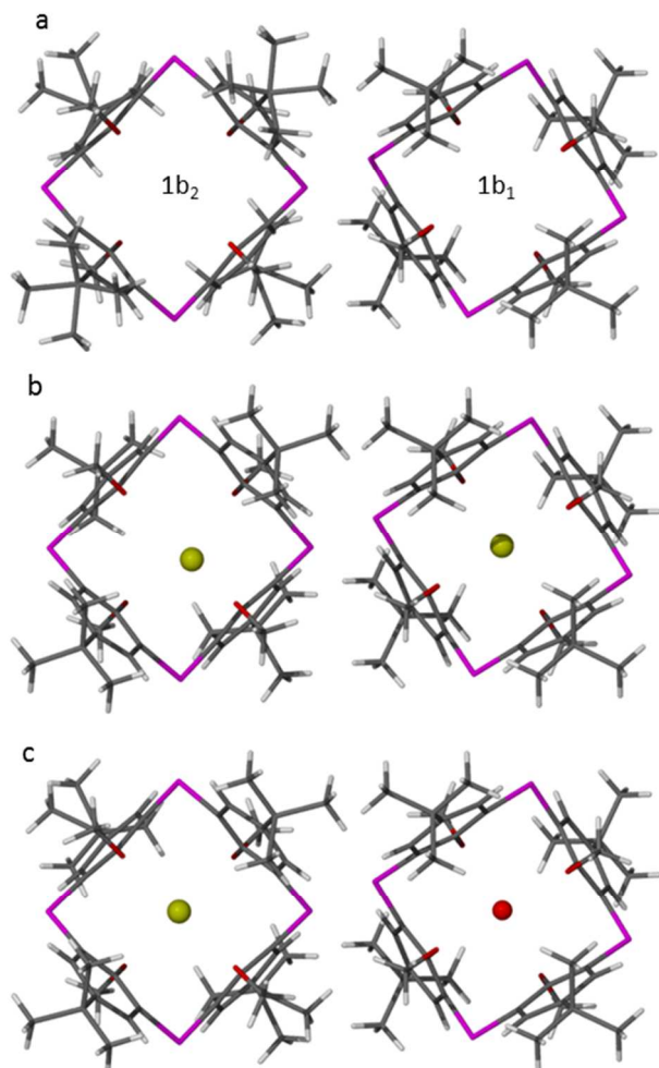
Fig. 2 Calixarene molecules in the structures of (a) \mathbf{1b} , (b) \mathbf{1b}_{\text{HCl}} and (c) \mathbf{1b}_{\text{HCl}\cdot\text{H}_2\text{O}} viewed along [001]. Symmetry-imposed disorder has been suppressed
