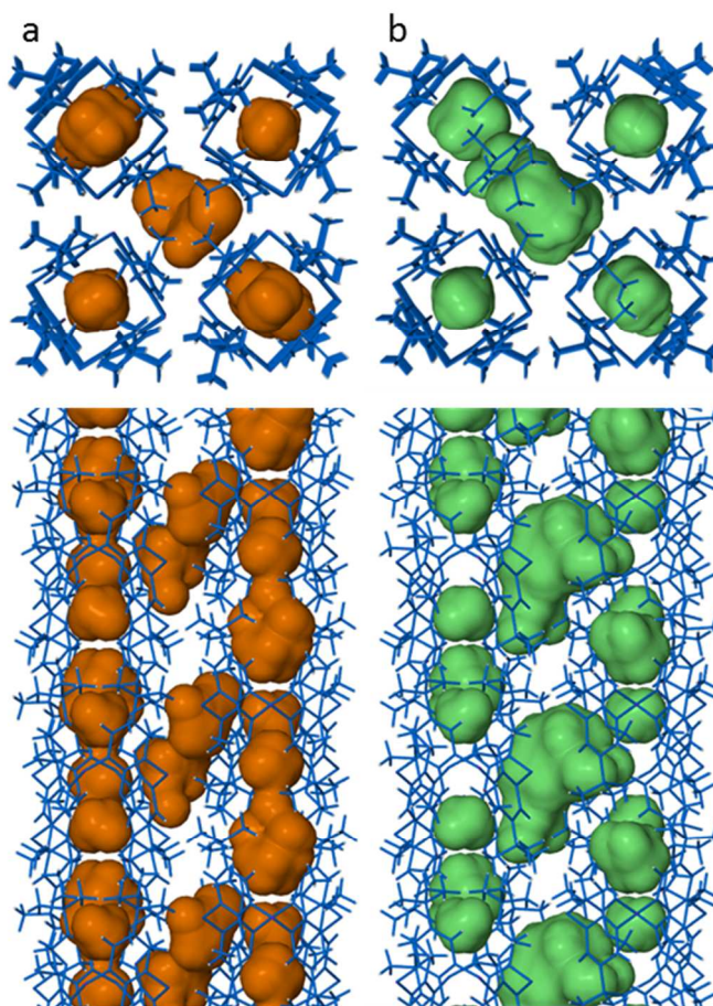
Fig. 4 Connolly surfaces of endo and intermolecular pores of calixarenes (a) 1b and (b) 1b 12 viewed along to [001] (top) and [110] (bottom). Symmetry-related disorder and the I 2 guest have been suppressed for clarity. Connolly surfaces have been generated using a probe radius of 1.2 Å.
