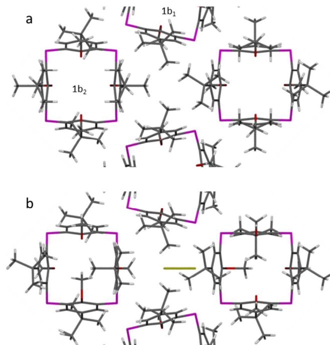
Fig. 3 Corresponding structures of (a) \mathbf{1b} and (b) \mathbf{1b}_{\text{I}_2} viewed along [001]. Symmetry-imposed disorder has been suppressed for clarity.
