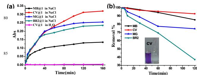
Fig. 4 (a) The dye release from dye@ 1 in a saturated NaCl aqueous solution and deionized water monitored at dye's UV-Vis absorption maximum. (b) Time depend chromatographic column efficiency determined by the absorbance before and after passing the column.
