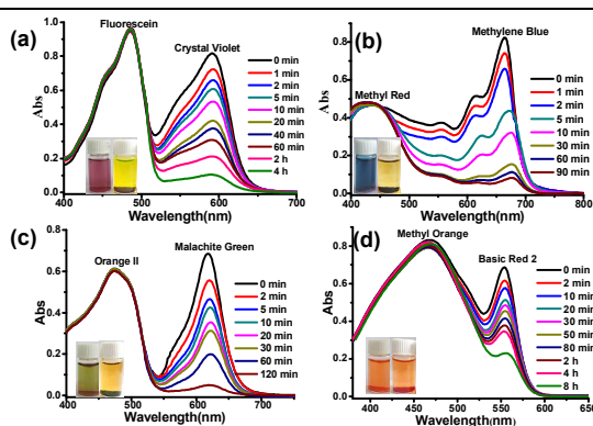
Fig. 3 UV-Vis spectra changes of 10.0 ml 8.0 ppm dye mixture in the presence of 20 mg 1 . (a) CV & Fluorescein ; (b) MB & MR ; (c) MG & Orange II and (d) BR2 & MO . The inset photographs are before (left) and after adsorption (right).
