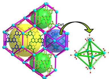
Fig. 2 (a) The large truncated octahedron (T-O h ) cage (left), small truncated tetrahedron (T-T d ) cage (middle) and medium cuboctahedron (cub-O h ) cage (right) of 1 . (b) 3D rht network (left) and six [Co(H 2 O) 6 ] 2+ arranged in a regular octahedron in medium cage (right) of 1 . Different color represents different TATAT 6- ligands.
