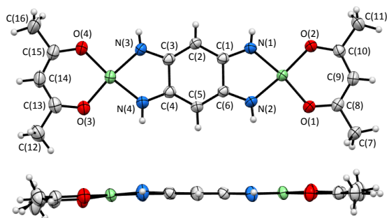
Fig. 2 Structure of 7 (anisotropic displacement parameters at 50%): top view and side view. Selected bond lengths ( \text{\AA} ): N(4)-C(4) = 1.319(3), C(4)-C(5) = 1.394(3), C(5)-C(6) = 1.393(3), C(6)-N(2) = 1.320(3), N(1)-C(1) = 1.318(3), C(1)-C(2) = 1.379(3), C(2)-C(3) = 1.386(3), C(3)-N(3) = 1.316(3), C(1)-C(6) = 1.498(3), C(3)-C(4) = 1.494(3).
