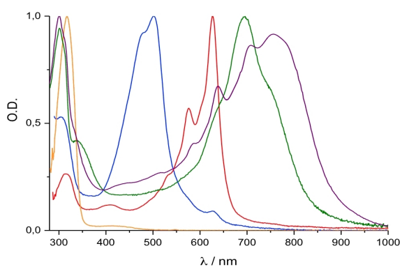
Fig. 3 UV-vis-NIR absorption spectrum of 2 and its oligomers. Colour code: 2 in \text{CH}_2\text{Cl}_2 (orange), 7 in \text{CH}_2\text{Cl}_2 (blue), 8 in THF (red), 10 in \text{DMSO} (green)* and 9 in \text{DMSO} (violet)*. (*) derived from a mixture in solution.
