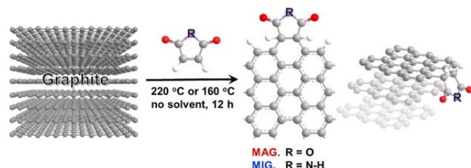
Scheme 1. a) Schematic representation of the solvent-free Diels-Alder reaction of graphite in the presence of a specific dienophile, maleic anhydride (MA) or maleimide (MI). The red spheres denote the oxygen.
