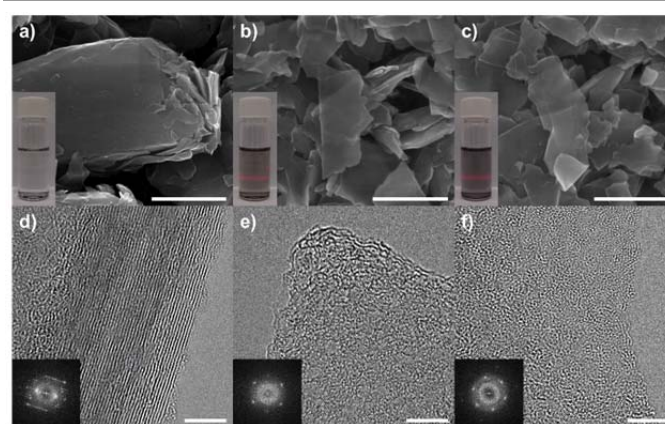
Fig. 1. SEM images: a) pristine graphite, b) MAG, and c) MIG. Scale bars are 1 \mu\text{m} . Insets in each case are photographs of the sample dispersion in NMP after standing for 1 month under normal laboratory conditions. The concentration is 0.5 mg/ml. HR-TEM images: d) pristine graphite, e) MAG, and f) MIG. Scale bars are 5 nm. Insets are SAED patterns of each respective sample.
