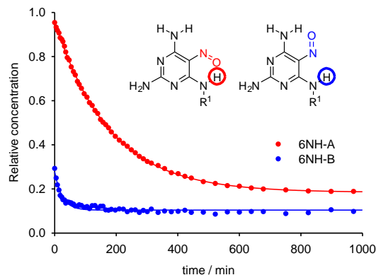
Fig. 6. The progress of the H/D exchange of hydrogen atoms of the amino group in position C6 in the equilibrium mixture of rotamers 1A and 1B in DMSO- d_6 -CD 3 OD mixture (9:1).
