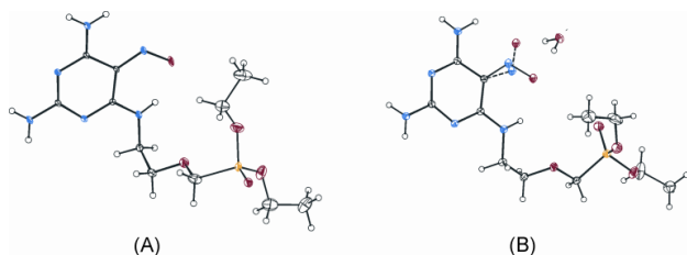
Fig. 4. X-ray crystallographic analysis of pure rotamer 1A (A) and of the monohydrate of compound 1 (B). Carbon is shown in grey, nitrogen in blue, oxygen in red and phosphorus in yellow. The less occupied position of nitroso group of rotamer 1B is drawn with dash lines (B). The displacement ellipsoids are drawn at a 30% probability level. The disordered atoms of the phosphonate moiety and solvating water molecule are omitted for clarity.
