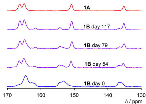
Fig. 3. Aromatic region of 13 C CP-MAS solid-state NMR spectra of planar rotamers 1A and 1B . Solid amorphous 1B slowly transforms into solid crystalline 1A . The full spectrum is available in Fig. S1 in ESI†.
