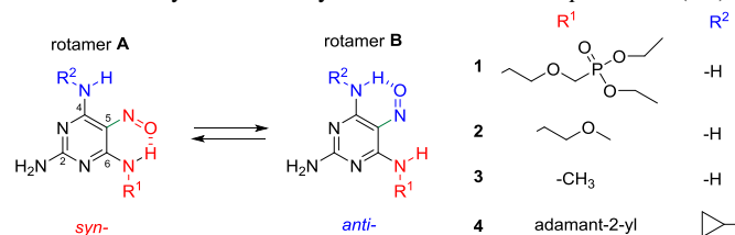
Fig. 1. Two possible geometries of the nitroso group in position C5 for compounds 1–4 . Rotamer A has a torsion angle C6-C5-N-O close to 0°; rotamer B has a torsion angle C6-C5-N-O close to 180°.
