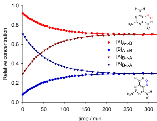
Fig. 5. Interconversion of rotamers 1A and 1B . Interconversion was monitored by 1 H NMR spectroscopy in DMSO- d_6 solution. R 1 = CH 2 -CH 2 -O-CH 2 -P(O)(OEt) 2 .
