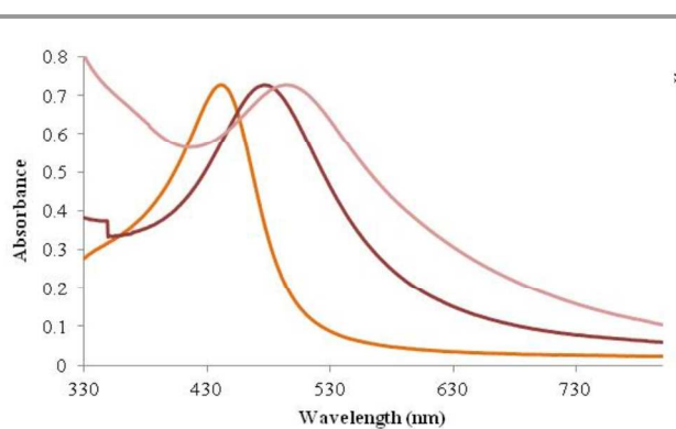
Fig 2 Comparison of the UV-Vis spectra of citrate-stabilised aqueous Ag-Au alloy NPs dispersed in water (orange-coloured trace), PS-SERS-NPs dispersed in THF (dark red-coloured trace) and the composite NPs dispersed in THF (pink-coloured trace).
