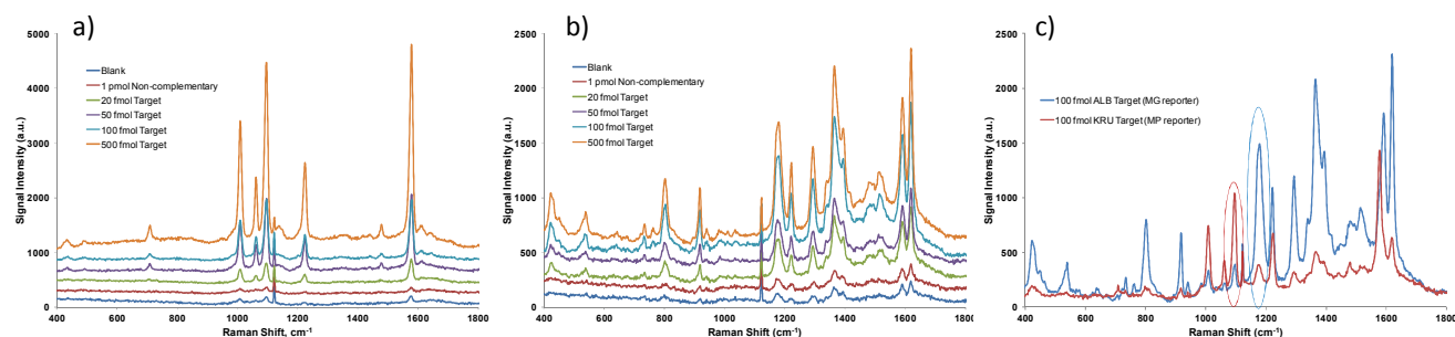
Fig. 3 Comparison of SERS spectra showing changes in signal intensity for a) MP measured for a range of C. krusei target concentrations; b) MG measured for a range of C. albicans target concentrations; and c) samples containing 100 fmol of either C. albicans or C. krusei target DNA (NP probes relating to both targets are present in both samples). Note, the sharp peak at \sim 1125 \text{ cm}^{-1} comes from the glass capillary tube.
