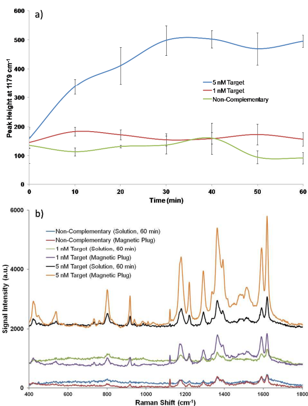
Fig. 2 Differences in MG signal intensity for samples containing either target or non-complementary DNA, showing a) change in peak height at 1179 \text{cm}^{-1} over 60 min for solution-based samples; and b) comparison of the SERS spectra for solution-based samples (after 60 min) vs. the magnetic plug of the same samples.
