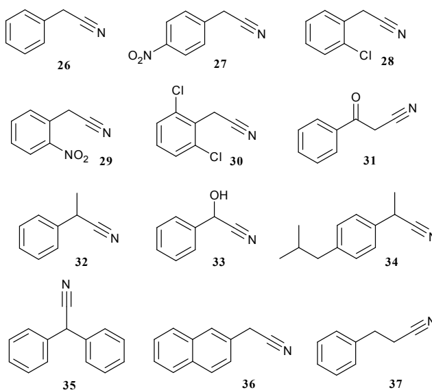
Figure 2. Nitrile substrates used to screen each nitrilase CFE.
