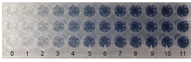
Figure 1. Reaction of OPA reagent with ammonia (concentration of \text{NH}_4\text{Cl} standard solution in mM indicated as number) after dilution with DMSO.
