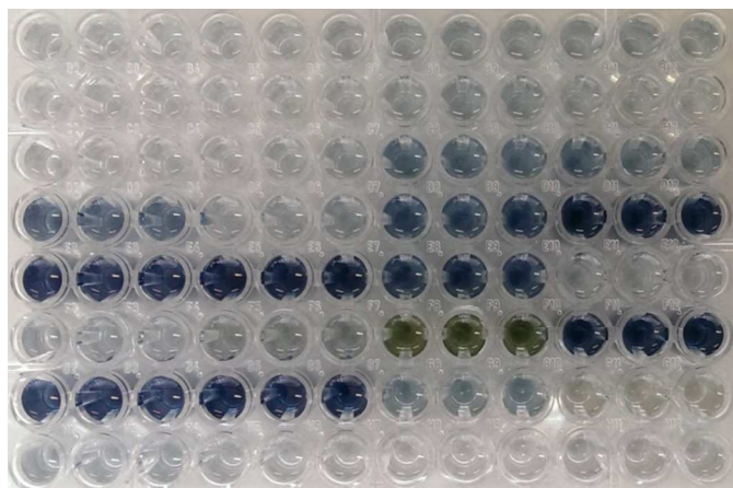
Figure 3. Reaction of OPA reagent with nitrilase 5 CFE solution after incubation with nitrile substrates 1-31 in triplicate (see fig. S2 for full details).
