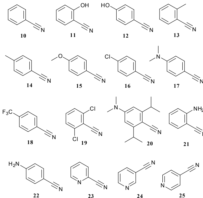
Figure 1. Reaction of OPA reagent with ammonia (concentration of \text{NH}_4\text{Cl} standard solution in mM indicated as number) after dilution with DMSO.
