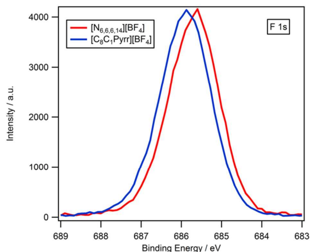
Figure 2. High resolution XP spectra of the F 1s region for [N_{6,6,6,14}][BF_4] and [C_8C_1\text{Pyrr}][BF_4] . Areas normalised to the area of F 1s photoemission peak for [N_{6,6,6,14}][BF_4] .
