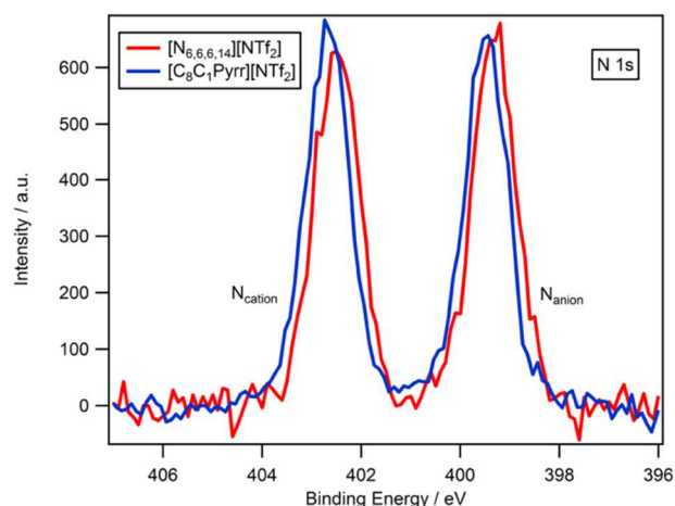
Figure 3. High resolution XP spectra of the N 1s region for [N_{6,6,6,14}][NTf_2] and [C_8C_1Pyrr][NTf_2] . Areas normalised to the area of F 1s photoemission peak for [N_{6,6,6,14}][NTf_2] .
