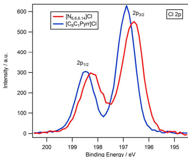
Figure 1. High resolution XP spectra of the Cl 2p region for [N_{6,6,6,14}]Cl and [C_8C_1\text{Pyrr}]Cl . Areas normalised to the area of Cl 2p photoemission peak for [N_{6,6,6,14}]Cl .
