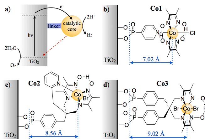
Figure 1. (a) Electron transfer processes in TiO 2 functionalised with a molecular catalyst for fuel production after UV-light excitation. The solid black and dashed red arrows indicate charge separation and recombination, respectively. Molecular structures of the catalysts for H + reduction are shown in (b) for Co1, (c) for Co2 and (d) for Co3 (charges omitted for clarity). The blue arrows indicate the distance between the anchoring groups and the catalyst metal centre ( r , Å), as determined by energy minimised DFT calculations (Figure S1). †
