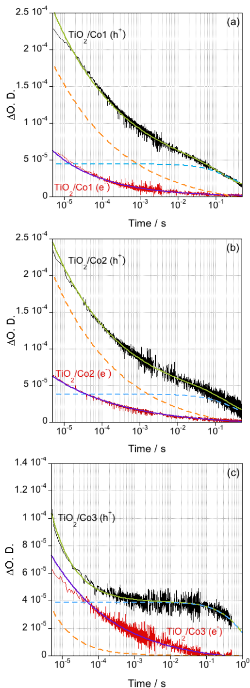
Figure 3. TA decays of TiO 2 loaded with (a) Co1, (b) Co2 and (c) Co3, measured in the absence of hole scavenger. The red traces correspond to electrons, while the black traces are assigned to holes. The orange and blue dashed lines represent the power law and exponential components of the biphasic holes decay, respectively.
