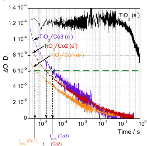
Figure 2. TA decays corresponding to photoexcited electrons in the TiO 2 for bare films (black trace) and when functionalised with Co1 (orange trace), Co2 (red trace) and Co3 (purple trace), measured in the presence of TEOA (0.1 M, buffered at pH 7) as hole scavenger.
