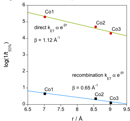
Figure 4. Plot of the logarithm of 1/t_{50\%} of the electron transfer from \text{TiO}_2 to the molecular catalyst (green trace) and the recombination between the reduced catalyst and the holes accumulated in the \text{TiO}_2 (blue trace) as a function of catalyst core-anchoring groups distance.
