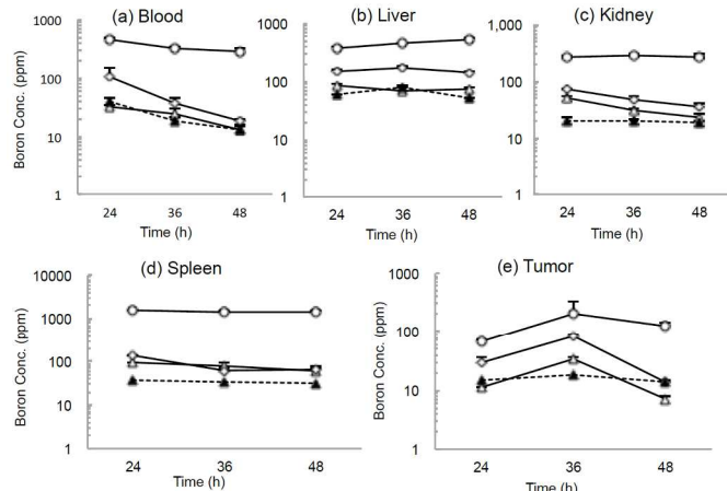
Fig. 4 Time courses of distribution of spd-BSH- and Na 2 B 10 H 11 NH 3 -encapsulating liposomes ( \Delta , spd-BSH: 15 mg[B]/kg; \diamond , spd-BSH: 30 mg[B]/kg; \circ , spd-BSH: 100 mg[B]/kg; \blacktriangle , Na 2 B 10 H 11 NH 3 : 15 mg[B]/kg). Each liposome was injected into tumor-bearing mice via the tail vein. Data are expressed as means \pm SD (n = 5).
