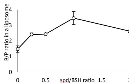
Fig. 2 Effect of amount of spd cation on spd-BSH encapsulation in liposomes. Boron/phosphorus (B/P) ratios of (spd) x closo -dodecaborate-encapsulating liposomes are shown in the vertical axis.
