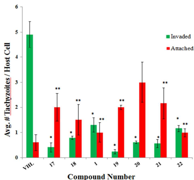
Figure 3. Quantification of invasion inhibition of nostodione A and mini panel using red/green assay. Compounds (20 \mu M) were tested for activity directly on extracellular tachyzoites using an established method. 12b Green bars represent invaded/intracellular parasites; red bars depict attached/extracellular parasites. Data are mean values \pm SEM of three independent experiments. *Tachyzoite invasion was significantly lower ( P \leq 0.05 , two-tailed Student's t -test) than the VHL control. ** Tachyzoite attachment to host cell was significantly decreased ( P \leq 0.05 , two-tailed Student's t -test) relative to VHL control.
