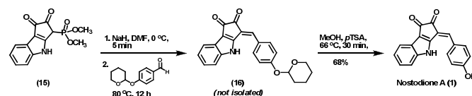
Scheme 2 Completion of the synthesis of nostodione A ( 1 ) employing the HWE strategy.
