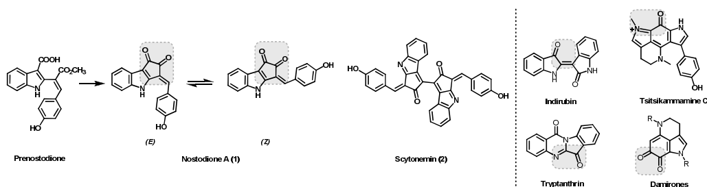
Figure 1 Structure of the cyanobacterial secondary metabolite nostodione A ( 1 ) and related biosynthetic alkaloids.
