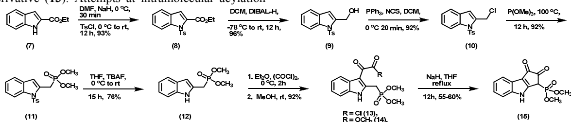
Scheme 1 Synthesis of the 3-oxalyl-indole-2-phosphonomethyl intermediates ( 13 ) and ( 14 ).
