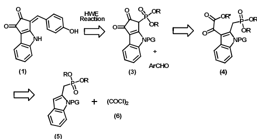
Figure 2 Retrosynthetic analysis of nostodione A ( 1 ).
