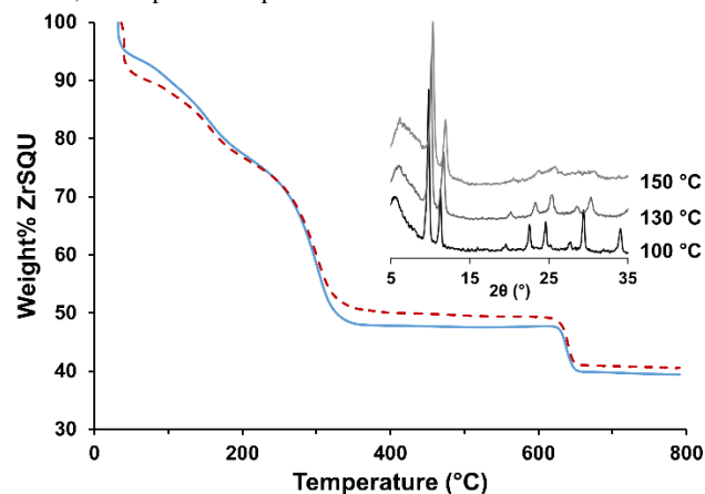
Fig. 4 TG profiles for as synthesized ZrSQU A (blue solid) and ZrSQU F (red dash) measured under \text{O}_2 . The framework loses long range order in the 130^\circ\text{C} - 150^\circ\text{C} range with a decrease in cell volume (inset).
