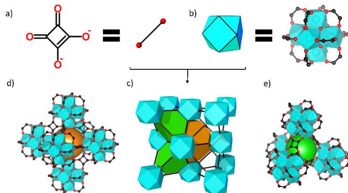
Fig. 1 Structural and topological representation of ZrSQU. SQU linkers (a) and Zr 6 O 4 (OH) 4 (C 2 O 2 ) 12 clusters (b) stack in an fcu-lattice (c), delineating octahedral (orange, d) and tetrahedral (green, e) cages with triangular windows. (Zr = blue; O = red; C = black).
