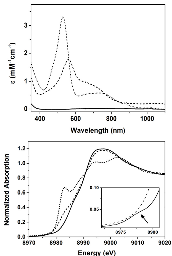
Figure 1. Top: Absorption Spectra of [\text{Cu}(\text{L1})](\text{BF}_4) ( 1 ) (dotted trace), and 2 (dashed trace) in \text{CH}_2\text{Cl}_2 at -90^\circ\text{C} ; Bottom: Normalized Cu k-edge spectra for [\text{Cu}(\text{L1})](\text{BF}_4) (dotted line), 1 (solid line), and 2 (dashed line). The inset depicts an expansion of the pre-edge region; the pre-edge of 1 is depicted by the arrow
