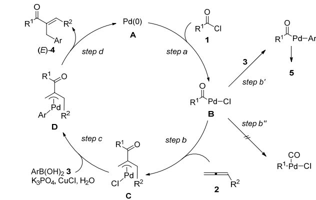
Scheme 1. Plausible mechanism.
