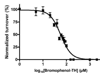
Fig. 5. DisA inhibition by bromophenol-TH. Assay was performed using \alpha - 32 P-ATP and TLC to monitor reaction progress. Reactions were stopped after 5 min and percentage of c-di-AMP was calculated. DisA activity was normalized with respect to the percentage of c-di-AMP formation in the absence of bromophenol-TH. IC 50 was measured as 56 \mu M.
