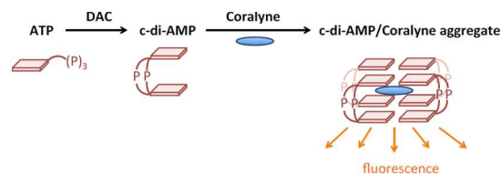
Fig. 2. Coralyne detection of c-di-AMP formation. 13 DAC converts ATP to c-di-AMP. Once c-di-AMP is formed, it can form complexes with coralyne. Iodide - in the solution quenches coralyne fluorescence in the absence of c-di-AMP. C-di-AMP protects coralyne from quenchers and c-di-AMP-coralyne complex's fluorescence can be detected.
