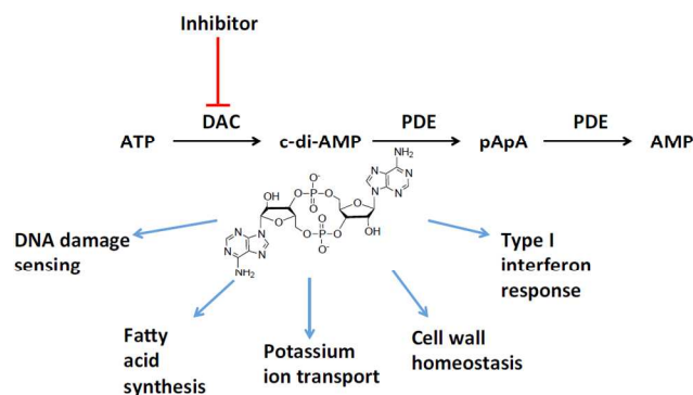
Fig. 1. Scheme of c-di-AMP signaling. Intracellular concentration of c-di-AMP is regulated by diadenylate cyclase (DAC) and phosphodiesterase (PDE). C-di-AMP affects many important cellular processes of bacteria as shown above.
