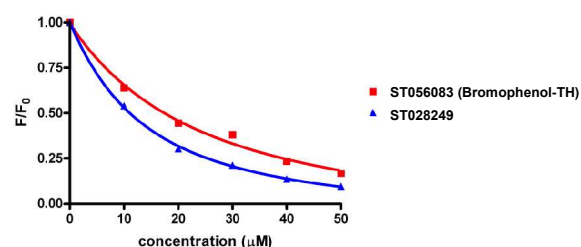
Fig. 4. Tryptophan fluorescence titration. Addition of small molecules to protein causes reduction of protein’s tryptophan fluorescence. Normalized fluorescence of ST056083 (bromophenol-TH) and ST028249 binding to DisA at 340 nm.
