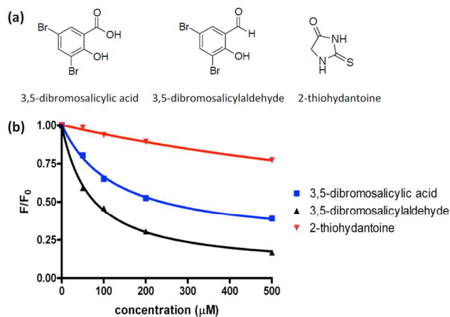
Fig. 7 (a) Structures of 3,5-dibromosalicylic acid, 3,5-dibromosalicylaldehyde and 2-thiohydantoin. (b) Normalized fluorescence at 340 nm of 3,5-dibromosalicylic acid, 3,5-dibromosalicylaldehyde and 2-thiohydantoin binding to DisA.
