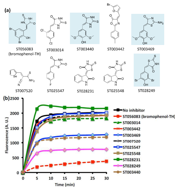
Fig. 3. (a) Structures of Bromophenol-TH and molecules in the 1000 compound library that have similar structures. (b) Real-time coralyne-based fluorescent detection of DisA reaction. 13
