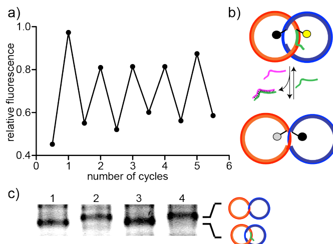
Figure 3 (a) Changes of the fluorescence intensity due to reversible catenane/pseudocatenane conversion. (b) Schematic for the toehold mediated switch. Addition of the TH-RO (green) leads to dehybridization of the rings and thereby the mobile state. Addition of the Comp-RO (pink), totally complementary to TH-RO reverses this process by forming the stable TH-RO/Comp-RO duplex. In the pseudocatenane state, the fluorescence is quenched due to close proximity between the fluorophore (Cy3, grey dot) and the quencher (BHQ-2, black dot). In the catenane state, dequenching of Cy3 (yellow dot) is observed. (c) Analytical agarose gel of the switching. Lanes 1 and 3 correspond to catenane, lanes 2 and 4 to pseudocatenane, respectively.
