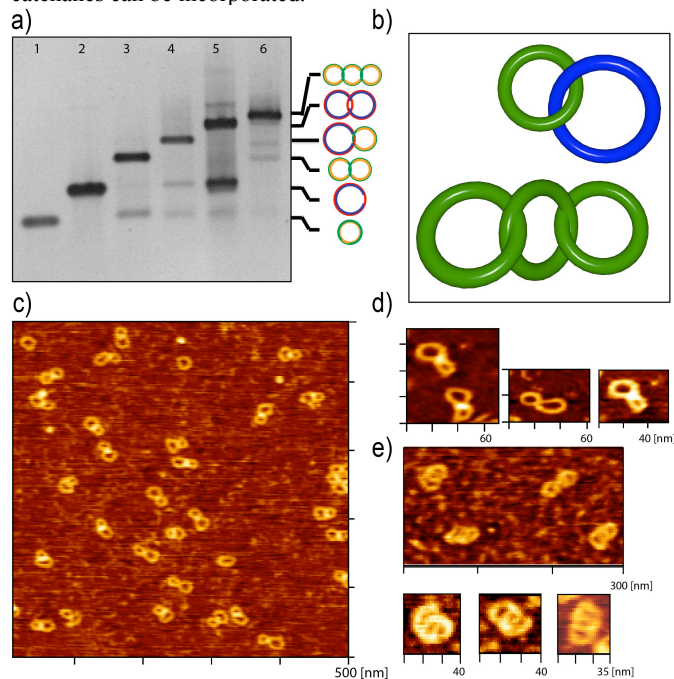
Figure 2 (a) Analytical agarose gel of the 126 bp ring (lane 1), the 168 bp ring (lane 2) and the catenanes containing two 126 bp rings (lane 3), one 126 and one 168 bp ring (lane 4), two 168 bp rings (lane 5) and the [3]catenane consisting of three 126 bp rings (lane 6). (b) 3D representation of how the asymmetric catenane and the [3]catenane arrange on the modified cationic mica surface for AFM. (c) AFM image of the non-symmetric catenane. 0.5 \mu\text{m}^2 area measured in intermittent contact mode in air. (d) AFM images (tapping mode in liquid) of these catenanes. The radii of rings were in agreement with the calculated ones (13.6 and 18.1 nm for the 126 and the 168 base pair rings, respectively). (e) AFM images of the [3]pseudo catenane (intermittent contact mode in air).
