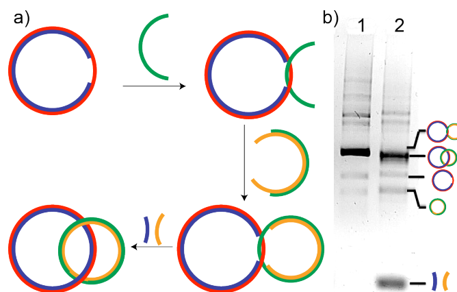
Figure 1 (a) Schematic of a non-symmetrical [2]catenane assembly. (b) Analytical agarose gel of the assembled non-symmetric catenane. Lane 1, pseudocatenane, lane 2, catenane after addition of RO's.
