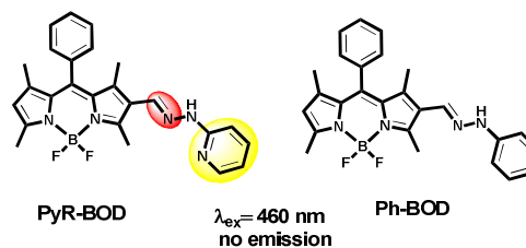
Scheme 2 Structure of probe and control probe
