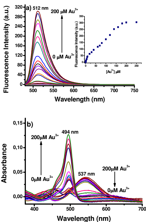
Fig. 1 (a) Fluorescence and (b) Absorbance spectra of PyR-BOD (10 \mu\text{M} ) in the presence of increasing amount of \text{Au}^{3+} (0–200 \mu\text{M} ) 0.1 M phosphate buffer/EtOH (pH 7.0, v/v, 1:1). Inset: Calibration curve. ( \lambda_{\text{exc}} : 460 nm at 25 ^{\circ}\text{C} ).
