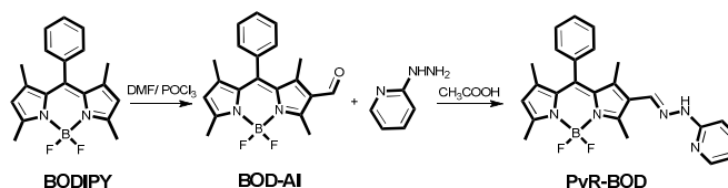
Scheme 1 Synthesis of probe
