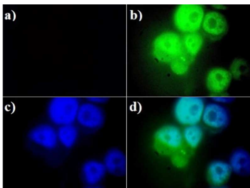
Fig. 2 Fluorescence images of Human Lung Adenocarcinoma cells (A549). (a) Fluorescence image of A549 cells treated with only PyR-BOD (5 μM); (b) Fluorescence image of cells treated with PyR-BOD (5 μM) and Au 3+ (10 μM) ( \lambda_{\text{ex}} = 460 \text{ nm} ); (c) Fluorescence image of cells treated with DAPI (control); (d) merged images of frames b and c.
