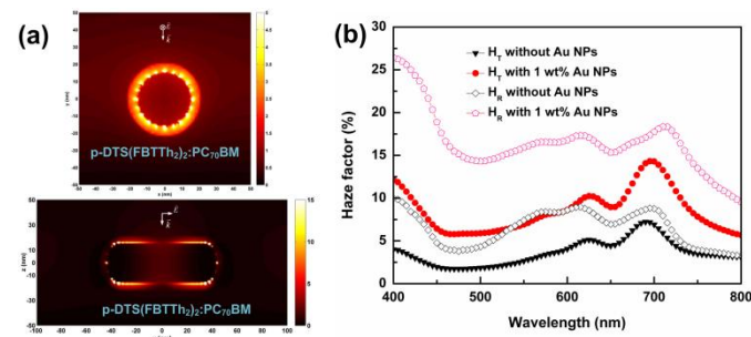
Fig. 3 (a) Electric field intensity distribution around Au-silica nanorods at 680 nm in side view and front view and (b) transmission and reflection haze factor spectra for p-DTS(FBTTh 2 ) 2 :PC 70 BM film with and without 1 wt% of Au nanorods.
