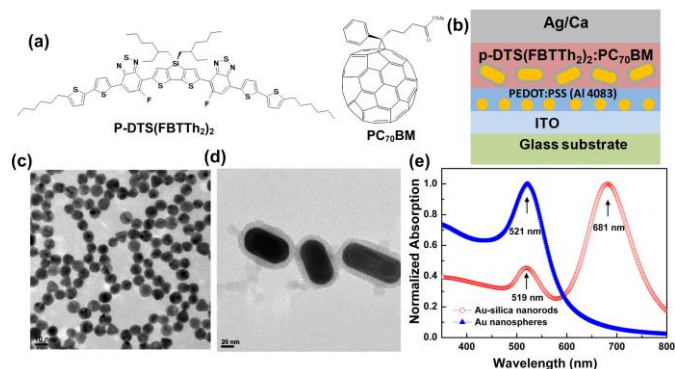
Fig. 1 (a) Molecular structures of the p-DTS(FBTTh 2 ) 2 and PC 70 BM, (b) device structure of the SM solar cell, (c) TEM image of Au nanospheres, (d) TEM image of Au-silica nanorods and (e) normalized UV-Vis absorption spectra of Au nanospheres in water and Au-silica nanorods in CB.
