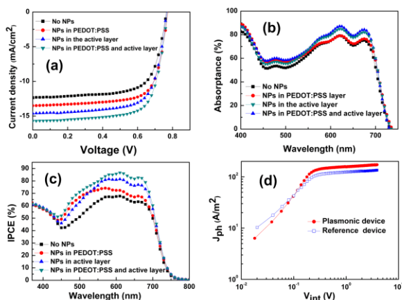
Fig. 2 (a) J - V characteristics of solar cells with and without the optimized concentration of NPs, (b) UV-Vis absorption spectra of p-DTS(FBTTh 2 ) 2 :PC 70 BM BHJ films with and without NPs, (c) IPCE spectra of solar cells with and without NPs and (d) photocurrent density ( J_{ph} ) versus internal voltage ( V_{int} ) characteristics of the reference device and dual NPs device.
