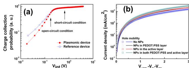
Fig. 4 (a) Charge collection probability ( P_C ) versus internal voltage ( V_{int} ) characteristics of the reference device and dual NPs device and (b) the dark J - V characteristics of hole-only devices with and without Au NPs.
