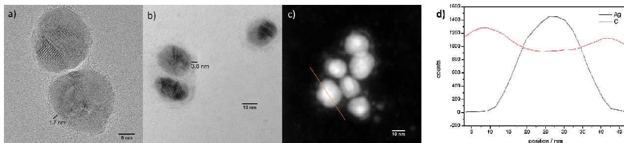
Figure 3. HRTEM image of a) PEG-coated Ag-NPs-3, b) pCBMA-coated Ag-NPs-4. c) EDXS line scan (orange) of pCBMA-coated Ag-NPs. d) C and Ag peak intensities along the EDXS line scan showing the Ag-pCBMA core-shell structure. The counts of C and Ag are plotted against the position. The core is close to 20 nm and the shell approx. 4 nm in size.
