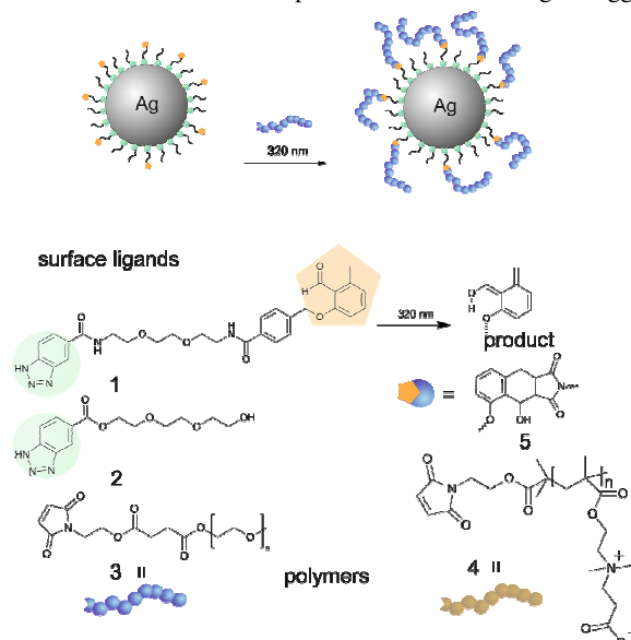
Figure 1. Light induced functionalization of Ag NPs with polymers. The novel photoactivable linker 1 and the inert linker 2 are attached to the Ag NP surface. 1 enables the light-induced cycloaddition with either PEG-Mal 3 or pCBMA 4 upon UV-irradiation resulting in cycloadduct 5 .
