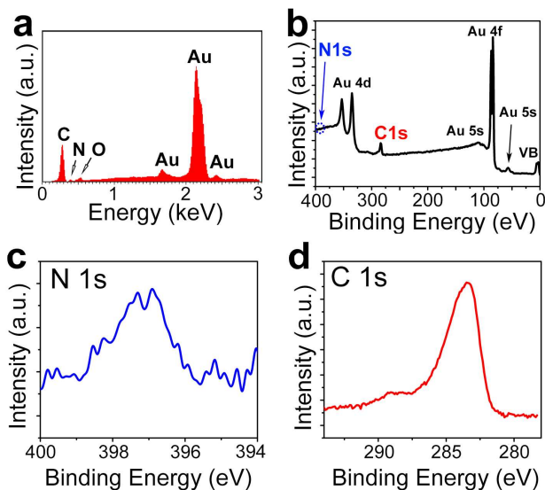
Fig. 4. Spectroscopic characterization of 4N-GNRs. (a) EDX spectrum of 4N-GNRs deposited on a gold substrate. (b-d) XPS spectra of 4N-GNRs deposited on a gold substrate: (b) survey spectrum, (c) N 1s spectrum and (d) C 1s spectrum.
