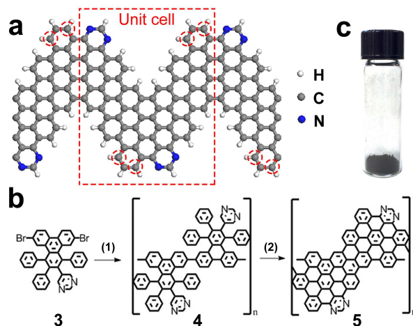
Fig. 1 Synthesis of 4N-GNRs. (a) Schematic of 4N-GNR. (b) Reaction scheme used in this work: (1) Yamamoto coupling, (2) Scholl reaction; see text and ESI for details. (c) Optical photograph of a 4N-GNR powder.
