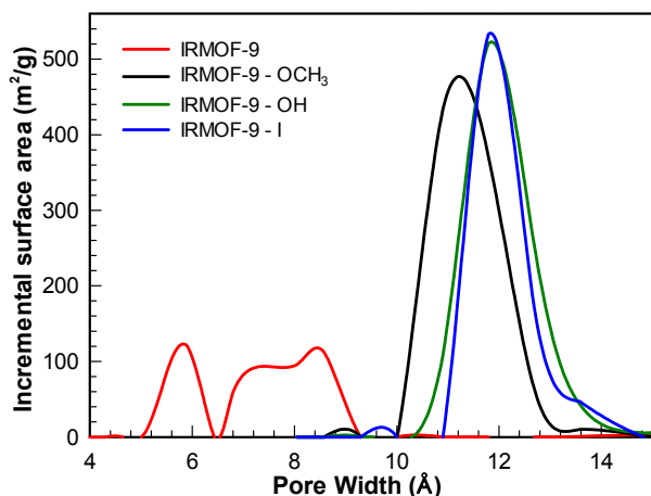
Fig. 3 Pore size distributions based on N_2 isotherms showing different pore sizes in IRMOF-9, but only one distinct pore in functionalised IRMOF-9 frameworks.
