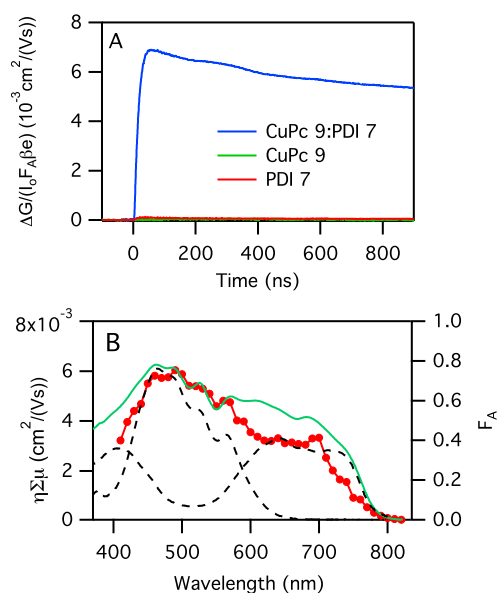
Fig. 4. (A) Photoconductance transients obtained upon excitation at 500 nm for pure PDI 7 , pure CuPc 9 and 50:50 (wt %) CuPc 9 :PDI 7 blend films. (B) The product of the yield per incident photon and the sum of the charge carrier mobilities (red, left axis) and the fraction of absorbed light ( F_A ) (green, right axis) in CuPc 9 : PDI 7 blend film as a function of the excitation wavelength. The scaled spectra of films of the individual compounds are also included.
