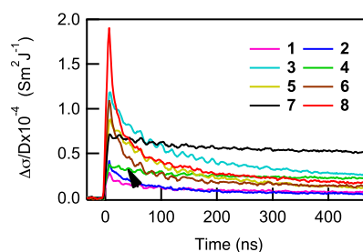
Fig. 3. Microwave conductivity transients of pure PDIs ( 1-8 ) obtained by exposing samples to 10 ns of 3 MeV electrons generated by a Van de Graaf accelerator.
