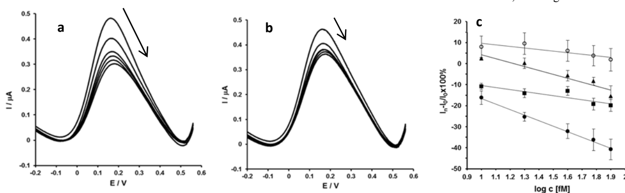
Fig. 2. Representative Osteryoung square-wave voltammograms (OSWVs; 1 mV, square-wave frequency: 50 Hz and amplitude: 25 mV) obtained for electrode modified with Co-porphyrin-ssDNA probe: 5'-APT TGG AGC TAT AGC AGG TT-3' (a) after hybridisation with 20-mer complementary ssDNA and (b) in the presence of sequence with three complementary bases at concentrations of 0, 10, 20, 40, 60 and 80 fM (buffer conditions: 0.09 M NaCl, 0.09 M sodium citrate, pH 7.0). (c) Relative intensity of redox Co(II)/Co(III) current vs log of concentration of 20-mer complementary ssDNA 5'- AAC CTG CTA TAG CTC CAA AT-3'; (●) sequence with three complementary bases: 5'- GGA GTT CTT CTC TCA TCA TC-3'; (■), sequence with one complementary base: 5'-GAA GAA GAG AGA GGA ACT CC-3'; (▲) fully non-complementary sequence: 5'-TTG GAC GAT ATC GAG GTT TA-3'.
