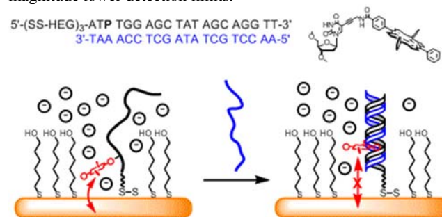
Scheme 1. Schematic illustration of signal generation mechanism of Co-porphyrin-DNA genosensor and sequences of the sensor and target strands (P denotes site of porphyrin modification).
