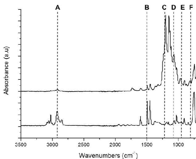
Fig. 3. ATR-IR spectra of the FS surface (top) and TCP (bottom) confirms the presence of both Si and F upon the FS surface. Stretching vibrations of the C-H bond are shown at positions A and B respectively, C-F vibrations (doublet) are shown at position C, stretching vibration involving Si are shown in positions D and E and the peak shown at position F is associated with the stretching of the Si-O-Si bond.
