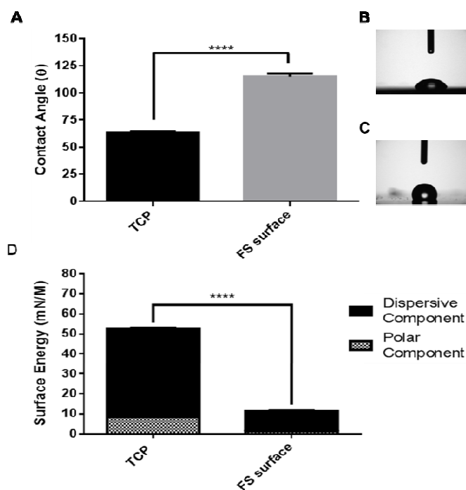
Fig. 2. Surface wettability is shown in A, with images of droplet spreading upon TCP and the FS surface shown in B and C respectively. Surface energy is shown in D (n=9).
