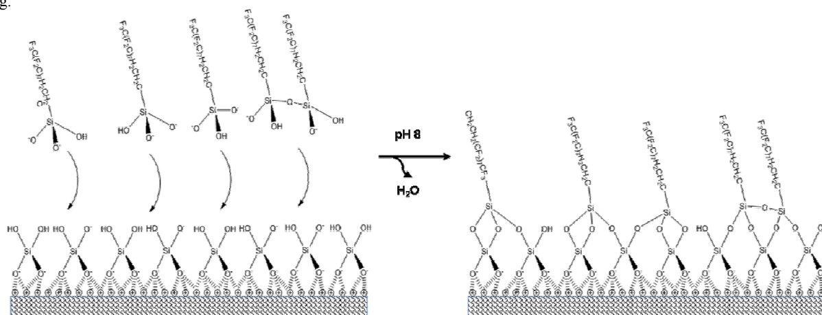
Fig. 1. Functionalisation of the silica film with FDTES via silanol group condensation. For simplicity the silica film is shown as a monolayer.
