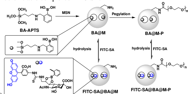
Scheme 1. Boronic acid-displaying MSN for intracellular delivery of FITC-SA. Sugar-laden MSN undergoes acidic pH promoted hydrolysis of boronate-diol ester.
