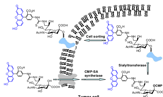
Fig. 1 Schematic for FITC-SA based tumor imaging. FITC-SA was preferentially uptaken into tumors and then incorporated into cellular proteins through endogenous sialylation pathway.
