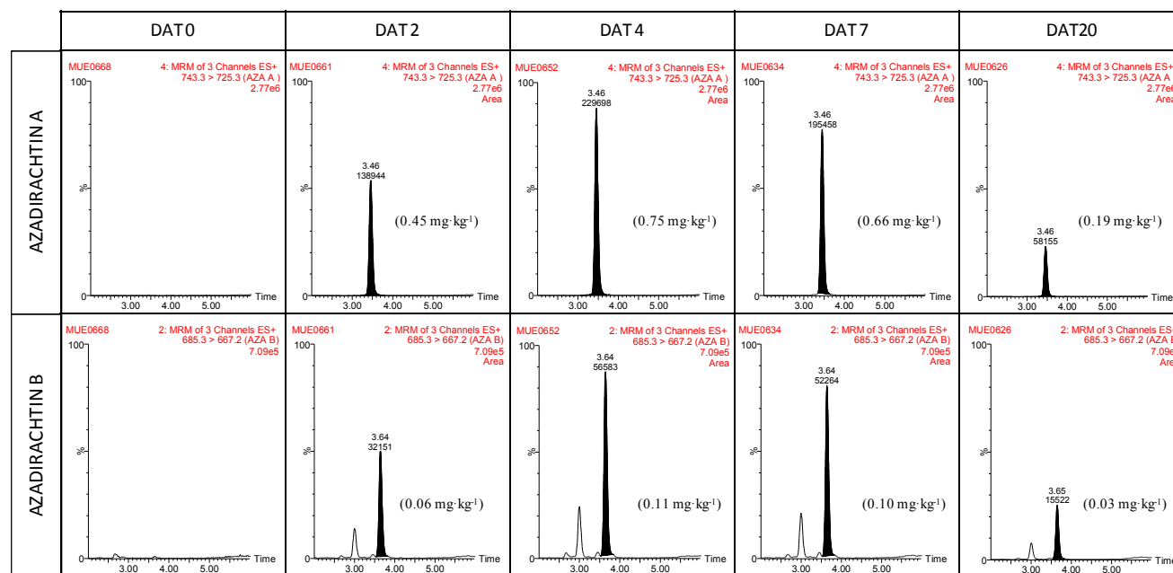
Fig.1. LC-MS/MS chromatograms (only Q transition is shown) for azadirachtin A and B in a Red/Freemani Maple Twigs sample collected at different days after application. Detected concentrations expressed in \text{mg}\cdot\text{kg}^{-1} are shown in brackets.
