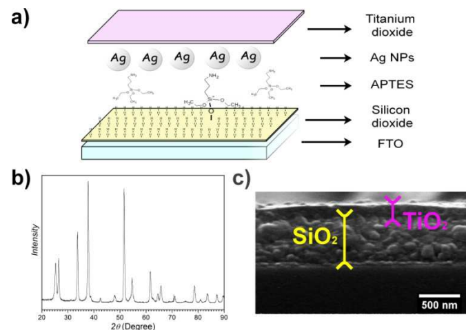
Figure 1: Device structure: a) schematic description of the architecture, b) X-ray diffraction pattern of the titania top layer and c) SEM cross section of the film.
