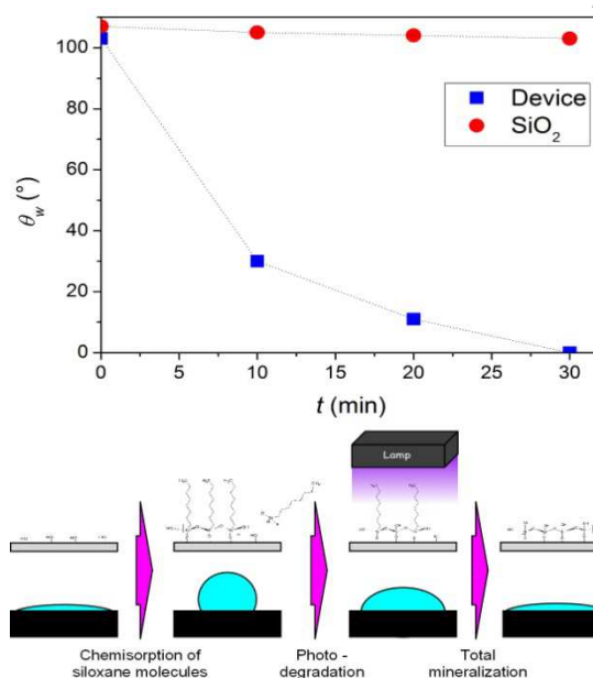
Figure 5. Kinetic of \theta_w decrease of the device covered by a chemisorbed siloxane layer under UV irradiation; scheme of the siloxane chemisorption and degradation.
