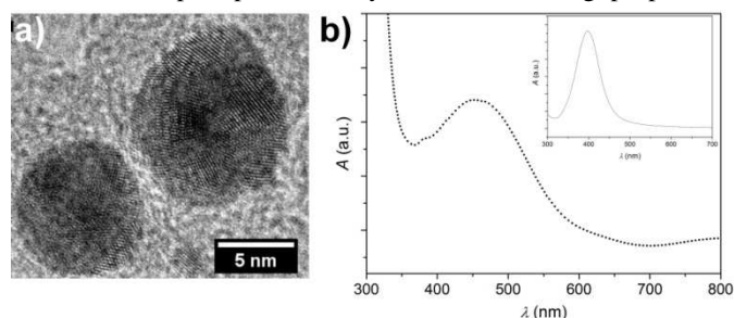
Figure 2: a) HR TEM picture of Ag NPs, showing high crystallinity and lattice spacing of about 230 pm; b) UV-Vis spectrum of Ag NPs grafted on the silica surface; inset: UV-Vis spectrum of the Ag NPs suspension.
