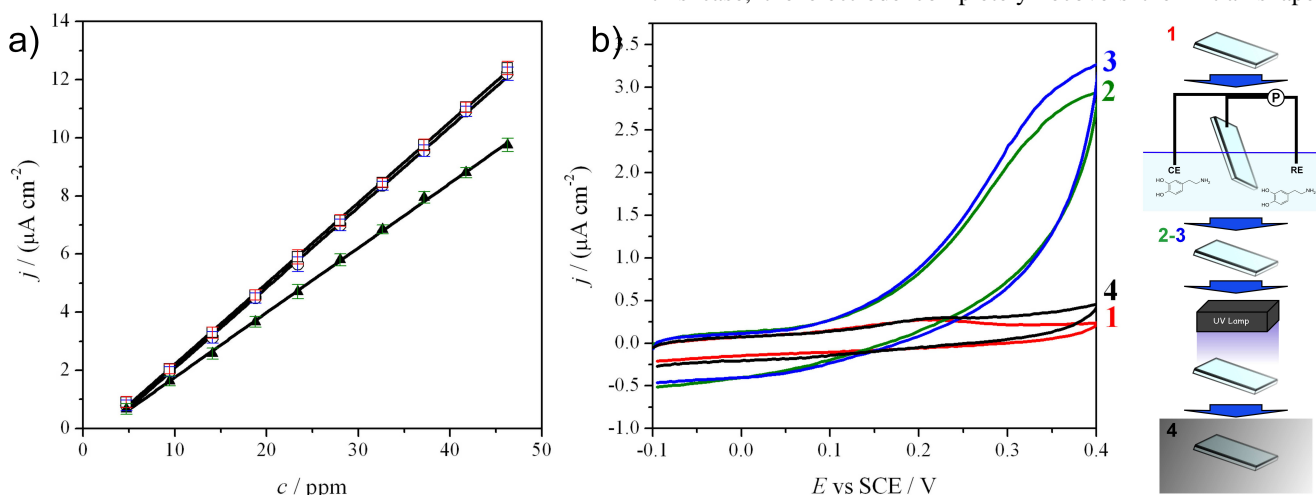
Figure 7. a) Dopamine calibration plots obtained at different analytical steps [squares (□): first calibration plot; triangles (▲): calibration plot after fouling; circles (○): calibration plot after UV cleaning]; b) Cyclic voltammograms registered at 0.1 V s -1 at different analytical steps during the fouling/cleaning procedure and relevant scheme.
