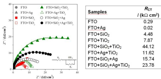
Figure 4: Complex plane plot spectra for all the electrode architectures, registered at +0.1 V (SCE) in the presence of the model probe molecule K_4[Fe(CN)_6] ; inset: equivalent circuit used to fit data. Table: charge transfer resistance ( R_{CT} ) values calculated from the fitting.
