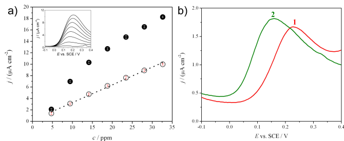
Figure 6. a) DPV calibration plots obtained for dopamine detection on two different electrode architectures (FTO+Ag+TiO 2 (●); FTO+SiO 2 +Ag+TiO 2 (○)); inset: differential pulse voltammograms referred to (○) data; b) differential pulse voltammograms, showing electrocatalytic peak displacement caused by Ag NPs (curve 1: FTO+SiO 2 +TiO 2 ; curve 2: FTO+SiO 2 +Ag+TiO 2 ).
