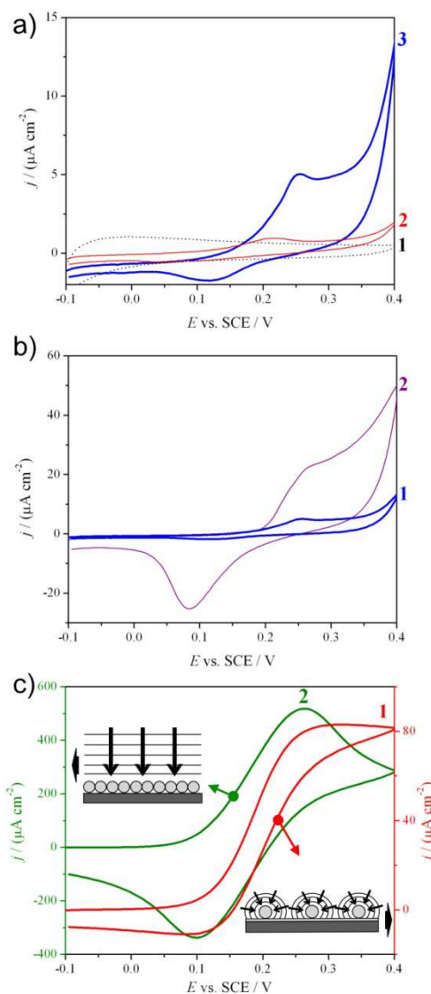
Figure 3: Cyclic voltammograms in the a,b) absence or c) presence of K 4 [Fe(CN) 6 ] probe molecule. Study of a) the effect of titania layer (curve 1: FTO+SiO 2 +TiO 2 ; curve 2: FTO+SiO 2 +Ag; curve 3: FTO+SiO 2 +Ag+TiO 2 ), b) the effect of silica layer (curve 1: FTO+SiO 2 +Ag+TiO 2 , curve 2: FTO+Ag+TiO 2 ), c) the distribution of Ag NPs (curve 1: FTO+SiO 2 +Ag; curve 2: FTO+Ag).
