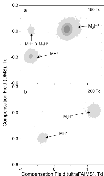
Fig. 9 Contour plots of ion intensity, compensation field in ultraFAIMS and compensation field in DMS for DMMP at 25°C with separation fields in ultraFAIMS of 150 Td (a) and 200Td (b) and the separation field in DMS of 50 Td for both plots
