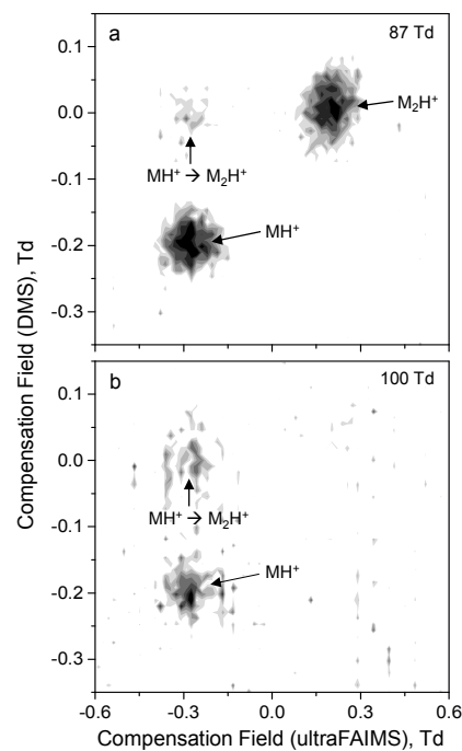
Fig. 5 Contour plots of ion intensity, compensation field in ultraFAIMS and compensation field in DMS for ethyl acetate at 40°C with separation fields in ultraFAIMS of 87 Td (a) and 100 Td (b) and the separation field in DMS of 40 Td for both plots.
