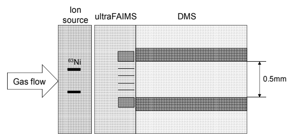
Fig. 1 Schematic representation of ultraFAIMS/DMS system
