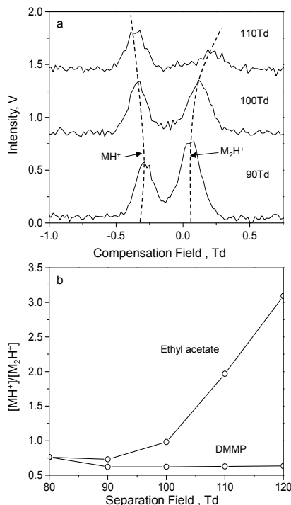
Fig. 4 Differential mobility spectra of ethyl acetate at 40°C for various separation fields in ultraFAIMS (a) and the change in monomer to dimer ion ratio for ethyl acetate and DMMP as a function of separation field strength (b)
