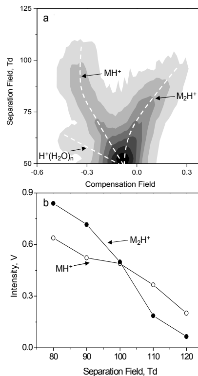
Fig. 3 Dispersion plot of ethyl acetate and the intensity of its monomer and dimer ions at 40°C in ultraFAIMS
