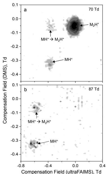
Fig. 6 Contour plots of ion intensity, compensation field in ultraFAIMS and compensation field in DMS for acetone at 40°C with separation fields in ultraFAIMS of 70 Td (a) and 87 Td (b) and the separation field in DMS of 40 Td for both plots
