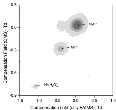
Fig. 2 Contour plots of ion intensity, compensation field in ultraFAIMS and compensation field in DMS for DMMP at 25°C with separation field in ultraFAIMS of 100Td and the separation field in DMS at 50 Td
