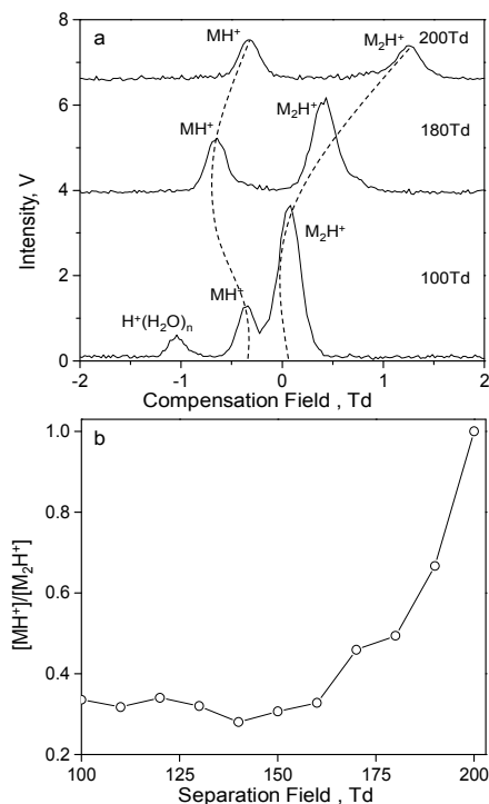
Fig. 8 Differential mobility spectra of DMMP at 25°C for various separation fields in ultraFAIMS (a) and the change in monomer to dimer ion ratio as a function of separation field strength (b)
