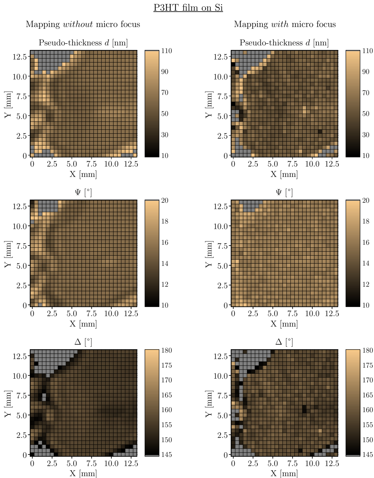
Fig. 5 Thickness, \Psi , and \Delta maps of a spin-coated P3HT film, measured at 65^\circ incidence angle. The 729 points were mapped in approximately 50 min. Areas with film thicknesses > 110 nm, \Psi > 20^\circ , and \Delta < 145^\circ are marked in grey, in order to better visualize the clear correlation between \Delta and thickness. \Psi and \Delta were mapped in 2 min and 23 min, respectively.
