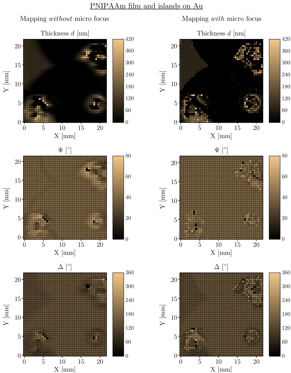
Fig. 4 Thickness, \Psi , and \Delta maps of a partly homogeneously and partly inhomogeneously PNIPAAm-covered gold substrate, measured at 65^\circ incidence angle. Homogeneously covered parts (upper-left areas) and three inhomogeneously covered “polymer islands” are well distinguishable in the micro-focus maps. \Psi and \Delta were mapped in 6 min and 59 min, respectively.
