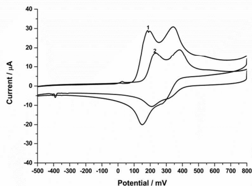
17 18 19 20 21 22 23 24 25 26 27 28 29 30 31 32 33 34 35 36 37 38 39 40 41 42 43 44 45 46 47 48 49 50 51 52 53 54 55 56 57 58 59 60 Fig. 4 Cyclic voltammograms of TMB (1) and oxidized TMB (2). The scan rate was 50 mV s -1 and 0.01 M PBS was added as counter electrolyte. The potentials were adjusted vs. Ag/AgCl RE.
