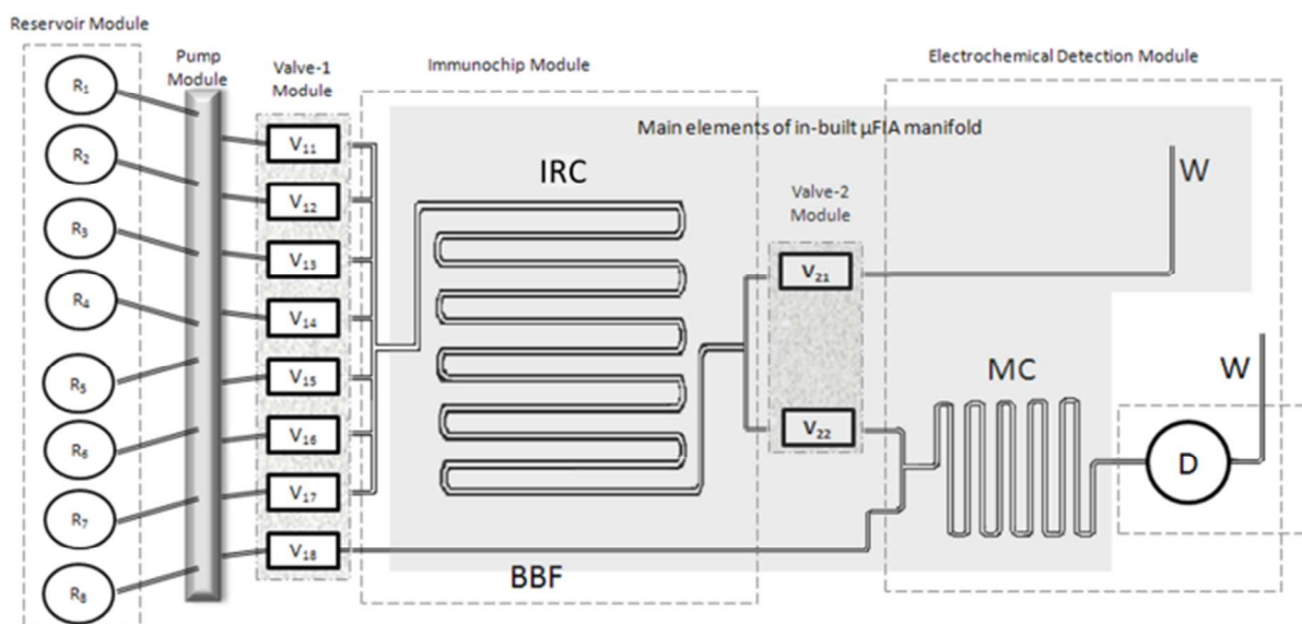
Fig. 2 A Schematic representation of \mu FIA BAM immunosensor constructed by interconnecting individual modules to facilitate different functions: Reagent reservoirs ( R_1 to R_8 ) for different solutions to be delivered sequentially into the immunoreaction chip (IRC). The fluidic operations we controlled by the miniaturized peristaltic micropump automated by LEGO® servo motors and valves (module 1: V_{11} to V_{18} ; module 2: V_{21} and V_{22} ). During assays, V_{18} provides a continuous flow of baseline buffer (BBF) from R_8 through the mixing chip (MC) to the detection unit (D). After immunoreaction, the contents of the channel in IRC are flushed either to the waste (W) or to D for detection using valves V_{21} and V_{22} . During detection, the electrochemically active substrate is mixed with BBF in MC and directed further to D where the amperometric peaks are recorded.
