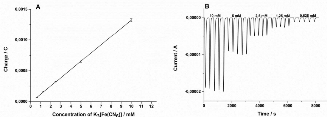
Fig. 3 (A) The linear relationship between the average peak areas in the amperometric recordings and concentration of K_3[Fe(CN)_6] injected into the detection chamber from the microchannel of IRC (injection loop) of the \mu FIA system. Five injections we made for each concentration; the error bars represent standard deviation. (B) A set of recorded reduction current peaks for each of the used concentrations of K_3[Fe(CN)_6] (in mM: 10, 5, 2.5, 1.25, and 0.625).
