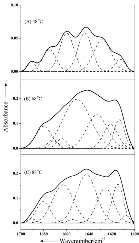
Fig.2 Deconvoluted ATR-FTIR spectra of the BSA solution in the amide I region together with the respective best-fitted individual band components at 48 °C (A), 68 °C (B), and 88 °C (C). Solid and dotted lines indicate the experimental data and the individual Gaussian components, respectively.
