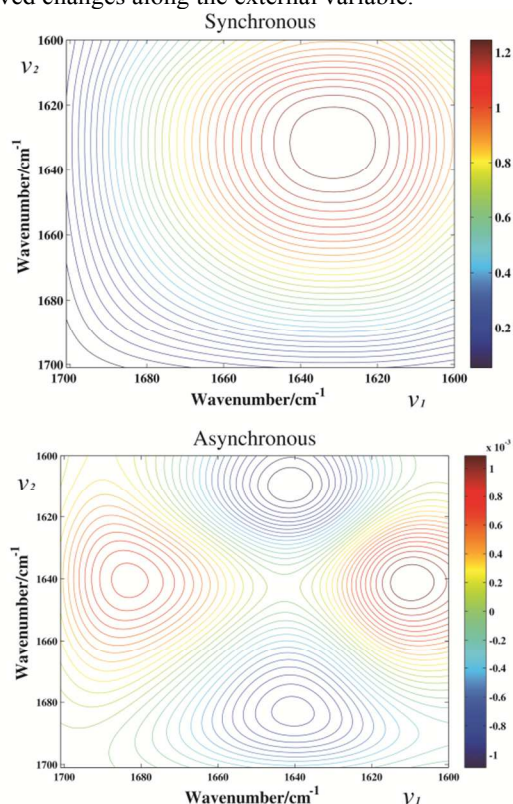
Fig. 4 Synchronous and asynchronous 2D ATR-FTIR correlation spectra constructed from 31 spectra recorded at 2 °C BSA during thermal transition from 30 to 90 °C.
