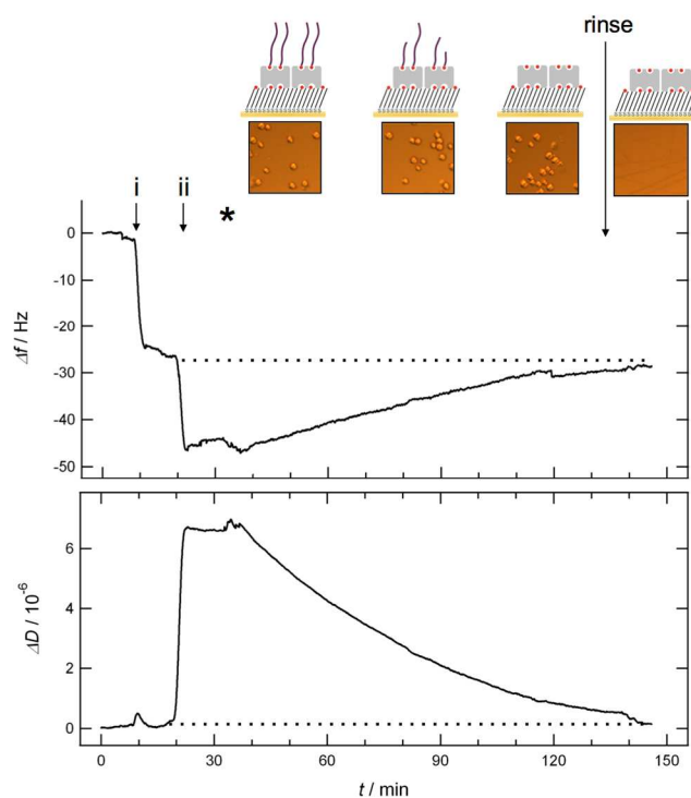
Figure 3. QCM-D frequency ( \Delta f , middle row) and dissipation ( \Delta D , bottom row) shifts for the addition chondrocytes (marked by an asterisk) to immobilized HA. (i) addition of SA flowed by (ii) addition of HA. Top row: schematic illustration of the suggested degradation process and light microscopy images taken during the QCM-D experiment during incubation with cells and after rinsing with media.
