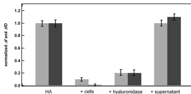
Figure 4. Normalized QCM-D frequency (light grey) and dissipation shift (dark grey) for a HA layer ( \Delta f and \Delta D for the HA layer is set to 1) and after the subsequent addition of either cells, hyaluronidase (data taken from Ref. 6) or supernatant.
