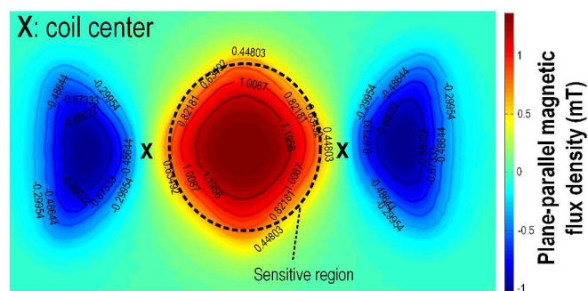
Fig. 9 Plane-parallel magnetic flux density map of the 14-turn figure-8 shaped coil at z = 0.6 mm (depth of the ITO glass). The sensing region, which is defined as the area have a plane-parallel magnetic flux density larger than 50% its peak value (1.43 mT) is located between the centers of two coils and has a shape of circle with diameter around 4.2 mm.
