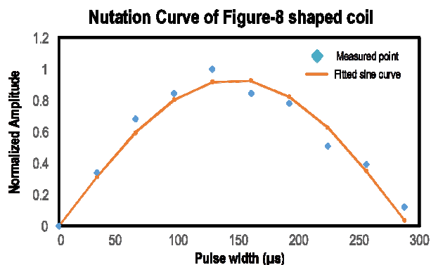
Fig. 4 Nutation curve of the 14-turn figure-8 shaped coil. The Normalized amplitude from different duration of RF excitation signals was recorded and fitted to the sinusoidal wave. The estimated \pi/2 pulse widths for the coil is 144 \mu\text{s} .
