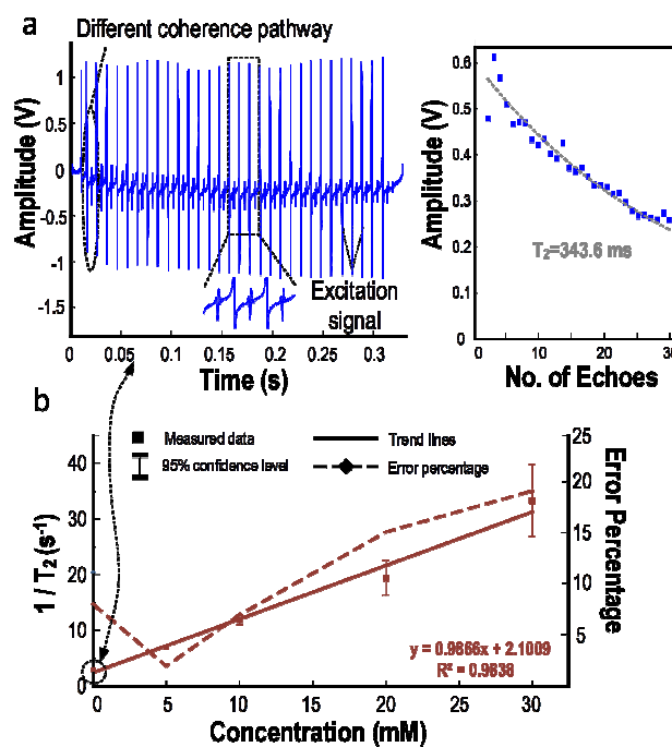
Fig. 5 (a) Received NMR signal from water. The received signal is composed by trains of echoes induced by the CPMG pulses. The glitches between the echoes are the excitation pulses. Usually the first echo is neglected for relaxation time derivation since it is interfered by different coherence pathway. Inset shows the enlarged received NMR signal. The echoes are clearly and their peak-to-peak amplitudes were plotted on the right against time, with a decreasing exponential manner, which was bounded by the grey dotted trend line. The derived relaxation time by the algorithm in this case is 343.6 ms. (b) Transverse relaxation time of the NMR signal versus concentration of \text{CuSO}_4 solution and results were shown on the graph (■). The trend lines were drawn together with their equation and R^2 value. 95% confidence levels were marked on the graph (—). In addition, the error percentages (defined as half of 95% confidence level/true value) are marked on the graph with dot lines where the values were displayed on the axis on the right.
