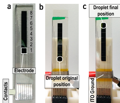
Fig. 7 (a) Fabricated DMF chip. For illustration, the electrodes are numbered 1-8; (b) and (c) Operation of the DMF platform. The droplet was originally placed at electrode no.1 (highlight by the circle). By applying signal on electrode no. 2 and then turn off electrode no. 1, the droplet moved to electrode no.2. As such, the droplet can be transported to electrode no.8, which is the NMR sensing site.
