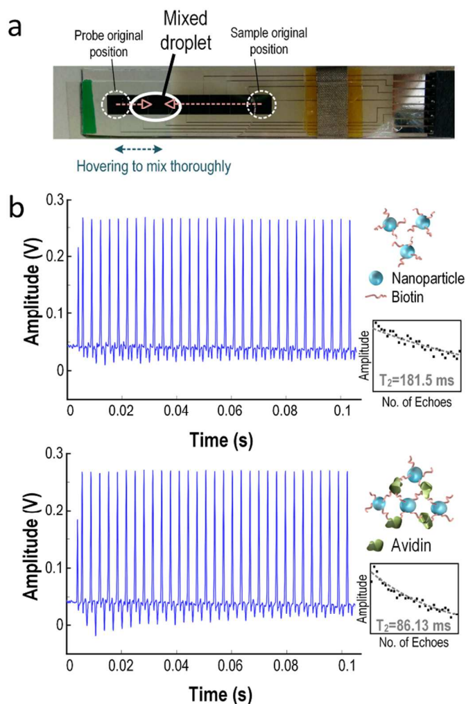
Fig. 8 (a) Illustration of droplets mixing. The droplets at electrode no. 1 (samples) and no. 8 (probe) were driven to electrode no.7 and mixed together. (b) The NMR assay results from the mixed droplets. Biotinylated magnetic nanoparticles acted as a probe. If the samples do not contain avidin, the nanoparticles will stay monodispersed and a longer T_2 will be obtained (181.5 ms). If avidin is with the samples, avidin and biotin will combine to form rigid bond and clusters will be presented. In consequence, T_2 will be decreased by the perturbation of the magnetic nanoparticle clusters (86.13 ms). This shows that the system is capable of detecting the existence of protein in the samples in a fully-automated way.
