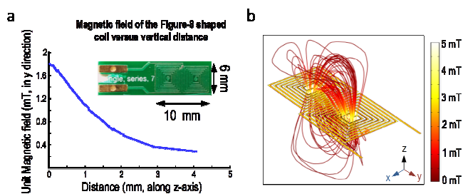
Fig. 3 (a) Plot of unit magnetic field in y-direction of the 14-turn figure-8 shaped coil along z-axis. The magnetic field is stronger on the coil surface (1.8 mT) and starts to decrease above the coil. Inset shows the photograph of the 14-turn figure-8 shaped coil; (b) The magnetic flux lines of the simulated 14-turn figure-8 shaped coil. The magnetic fluxes are still pointing in the z-direction at the centres of each coil. However, between the two coils, the magnetic flux is pointing in the y-direction, generating plane-parallel magnetic flux.
