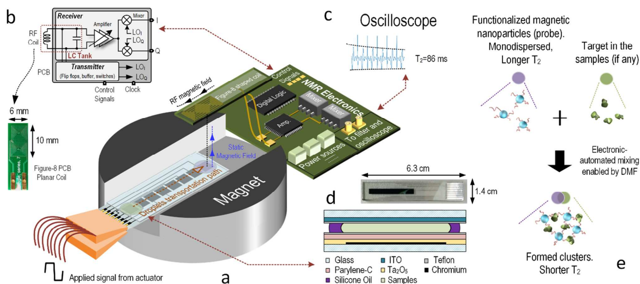
Fig. 1 The overall schematics and operations of the NMR-DMF system. (a) The placement of the DMF chip, magnet, RF coil and PCB board in 3D view. Benefit from the plane-parallel magnetic field generated by the figure-8 shaped coil, the NMR system can be effectively integrated into the DMF system; (b) Schematics of the NMR Electronics. The transmitter which is formed by the digital logics such as flip flops is used to excite the hydrogen atom. On the receiver part, the capacitor together with the RF-coil (fabricated figure-8 shaped coil) forms a LC tank to provide passive gain enhancing of the system's sensitivity. The signal is then amplified and down converted to f_{IF} (intermediate frequency) and fed to the external filters and oscilloscope; (c) The filtered results from the PCB are captured by the oscilloscope for easier demonstration purpose. Waveforms are then analysed and the spin-spin relaxation time ( T_2 ) is fitted by the algorithm written in MATLAB; (d) The photograph of the DMF chip and structure of the DMF platform. The droplets are squeezed between the top and bottom planes and surrounded by silicone oil; (e) The detection mechanism of the NMR-DMF system. The target-specific magnetic nanoparticles, which act as probes, are placed on the sensing site initially (in purple). The samples at other electrodes (in cyan) will be transported to the sensing site and mixed with the probes to perform NMR assays automatically by applying voltage on corresponding electrodes. Without the target, the probes stay monodispersed and will have a longer T_2 . Otherwise, the target and probes will form clusters by forming bonds between each other and the T_2 will be decreased.
