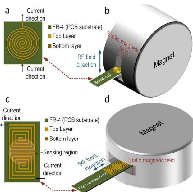
Fig. 2 (a) Illustration of a conventional spiral coil; the magnetic field generated by the current as shown in figure will have direction out of paper. The shape of the coil is typical circular to enhance the magnetic field at the center; (b) The placement of the magnet and the conventional spiral coil. Due to the fact that RF-field from the coil and magnetic field from the magnet have to be orthogonal to each other, the spiral coil and magnet must be configured as shown in the figure, which is not suitable for the DMF platform. (c) Illustration of the figure-8 shaped coil. Generally it is composed by two spiral coils in reversed direction (CW and ACW) in series and the field between two coils generated by the current shown in figure will have a direction pointing downward and it is the sensing region in our system. The shape of a single coil is square instead of circular to enhance the magnetic field at the sensitive region; (d) Placement of the magnet and the figure-8 shaped coil. Since the magnetic field goes parallel to the PCB substrate direction, the magnet and the coil now can be put as shown in the figure and the DMF platform can be effectively integrated with the NMR.
