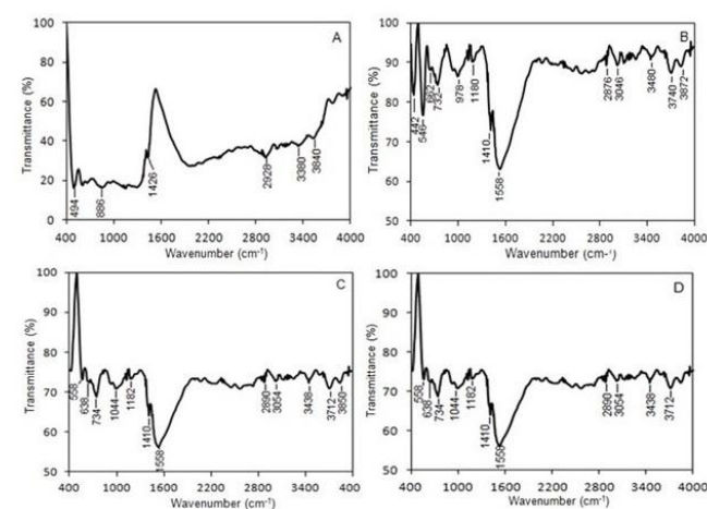
Fig. 4 FTIR transmission spectra of A) Bare Au, B) Au/MPA/PEI, C) Au/MPA/PEI-ssDNA and D) Au/MPA/PEI-dsDNA at frequency 400-4000 cm^{-1} .
