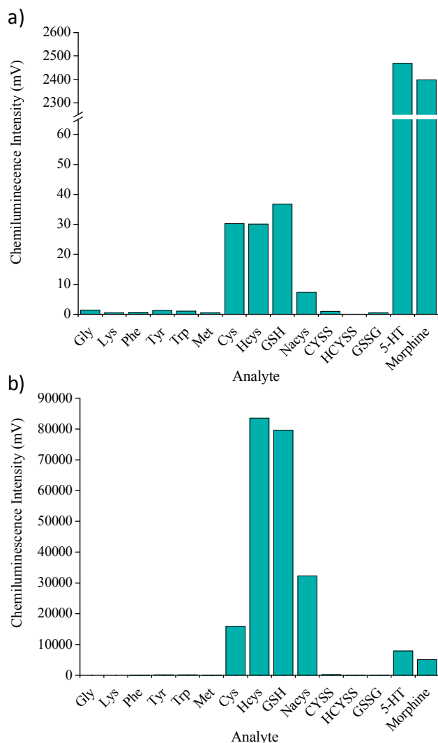
Fig 2 Chemiluminescence intensities for selected analytes ( 5 \times 10^{-6} M) with (a) acidic potassium permanganate ( 2.5 \times 10^{-4} M in 1% (m/v) sodium polyphosphate, pH 3) and (b) the permanganate reagent and formaldehyde, using flow injection analysis methodology.
